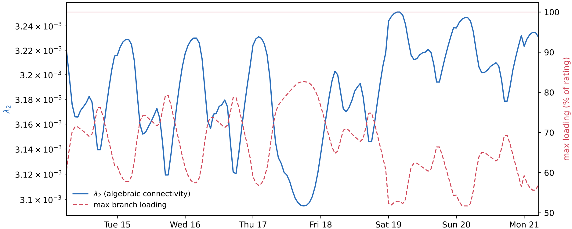
WP2024_all-island - headroom: how close the grid is to splitting, hour by hour
