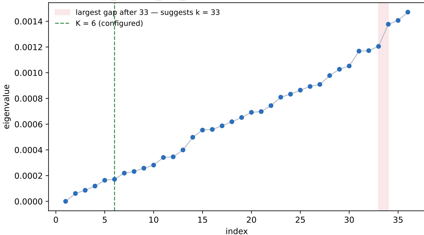
TYTFS2024_WP2024_V35_transmission +generators — sym, susceptance
