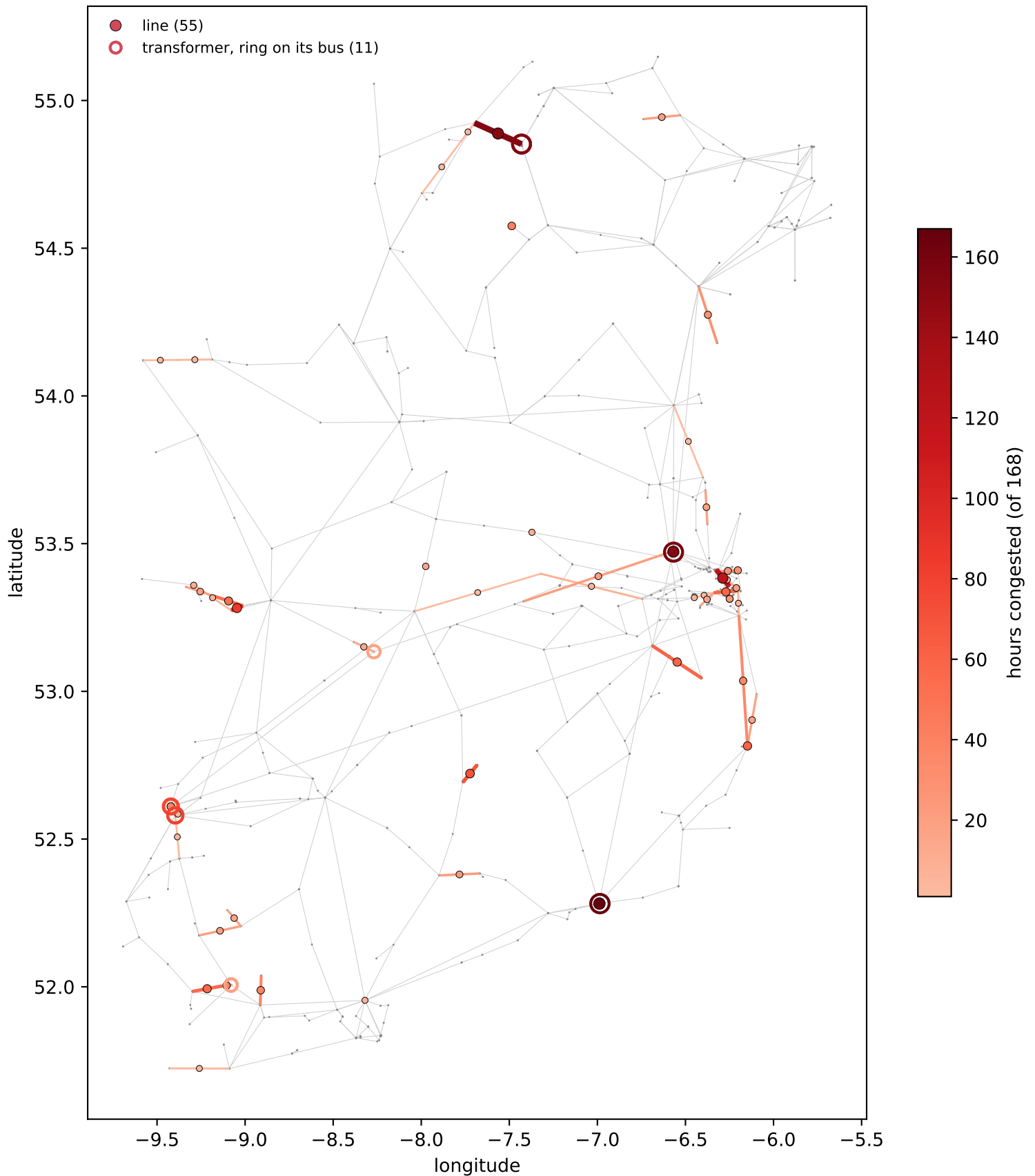
WP2033_all-island (capacity_constrained) - branches at \geq 70\% of rating, over 168 hours 66 of 980 branches congested at least once; 0 of them not placeable
