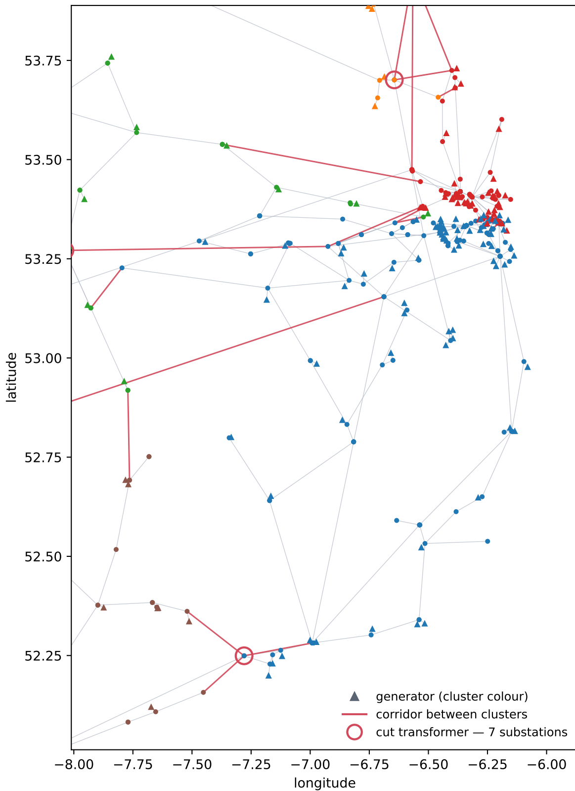
WP2024_all-island +generators — sym, headroom, k = 6, 2030-01-20 17:00:00 cluster 0 — 222 nodes
