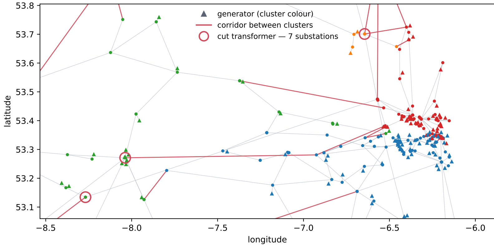
WP2024_all-island +generators — sym, headroom, k = 6, 2030-01-20 17:00:00 cluster 3 — 106 nodes
