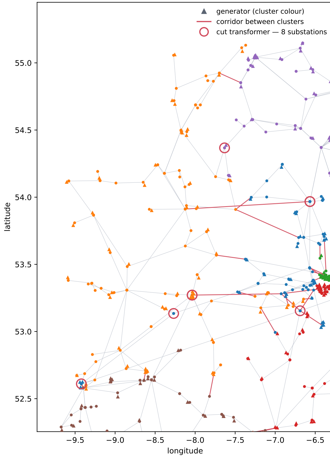
WP2024_all-island +generators — sym, loading, k = 6, 2030-01-20 17:00:00 cluster 1 — 188 nodes
