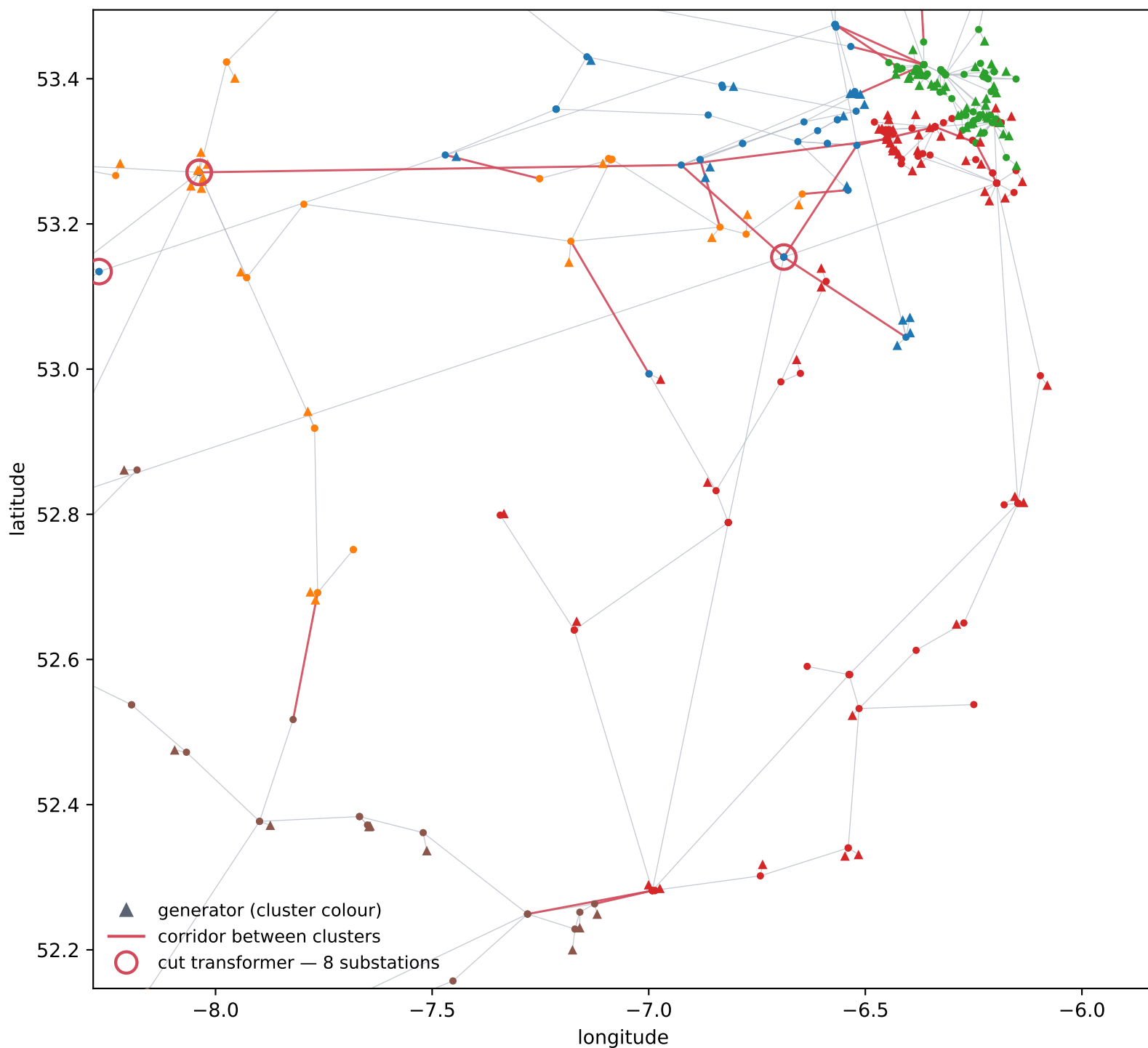
WP2024_all-island +generators — sym, loading, k = 6, 2030-01-20 17:00:00 cluster 3 — 141 nodes
