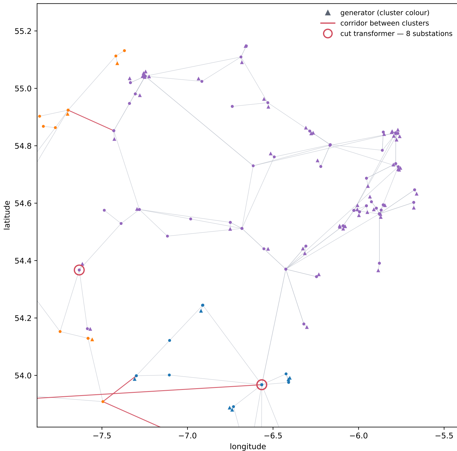
WP2024_all-island +generators — sym, loading, k = 6, 2030-01-20 17:00:00 cluster 4 — 176 nodes
