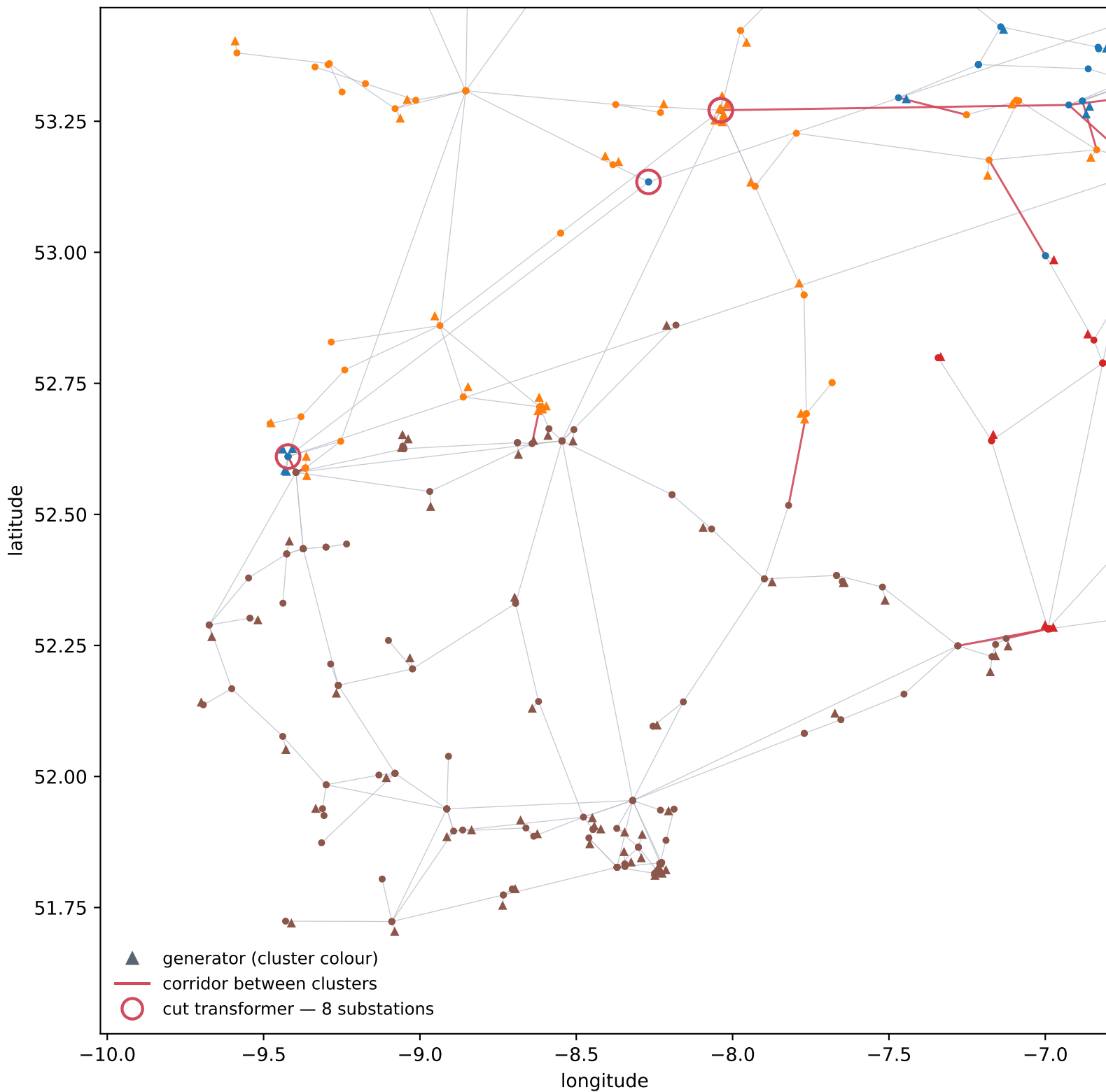
WP2024_all-island +generators — sym, loading, k = 6, 2030-01-20 17:00:00 cluster 5 — 204 nodes
