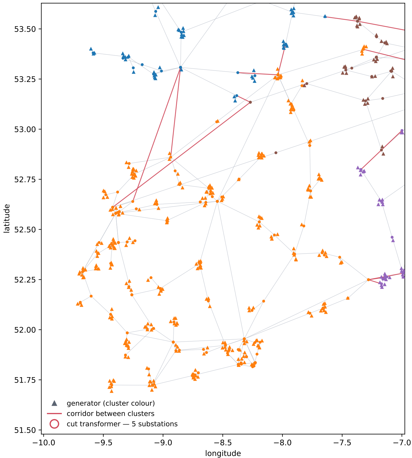
WP2033_all-island +generators — sym, headroom, k = 6, 2030-01-20 17:00:00 cluster 1 — 500 nodes
