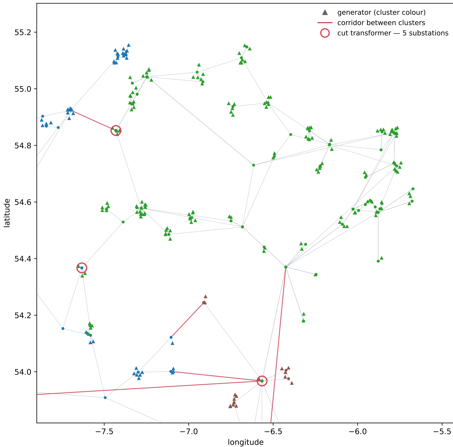
WP2033_all-island +generators — sym, headroom, k = 6, 2030-01-20 17:00:00 cluster 2 — 290 nodes
