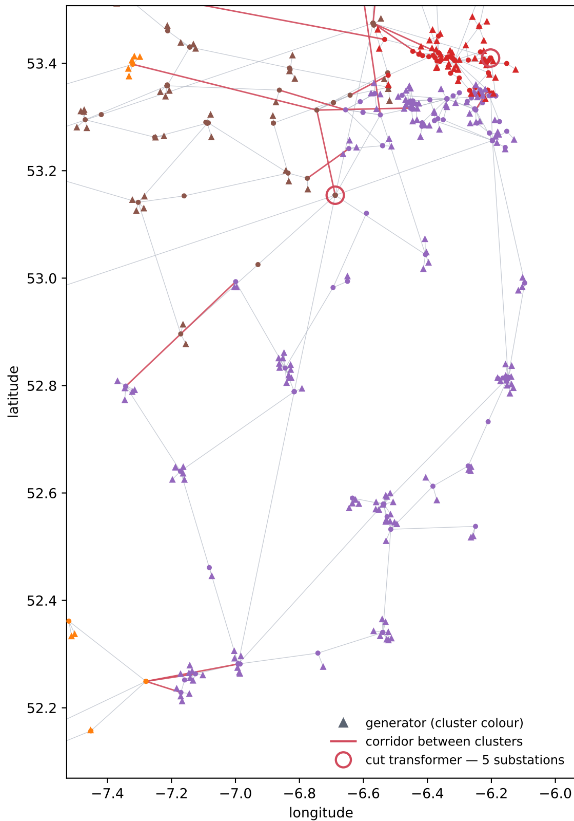
WP2033_all-island +generators — sym, headroom, k = 6, 2030-01-20 17:00:00 cluster 4 — 286 nodes
