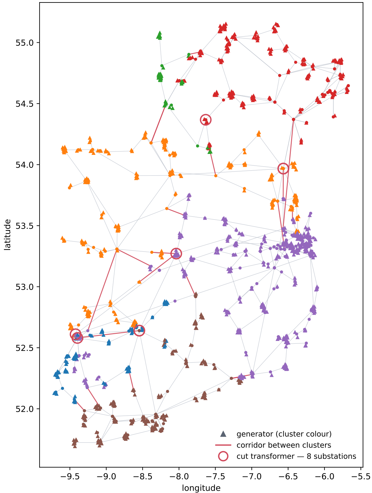
WP2033_all-island +generators — sym, loading, k = 6, 2030-01-20 17:00:00 751/751 buses placed, 39/1858 drawn corridors cut
