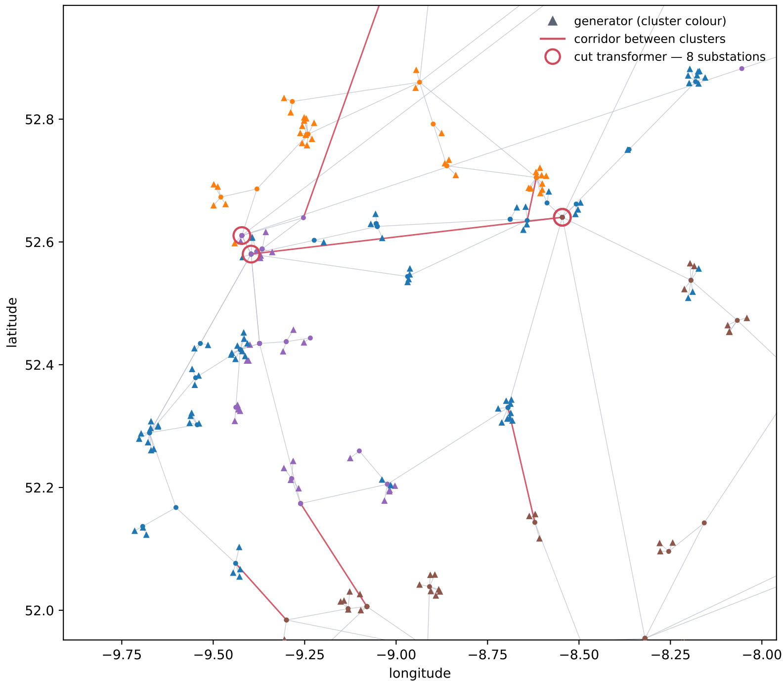
WP2033_all-island +generators — sym, loading, k = 6, 2030-01-20 17:00:00 cluster 0 — 113 nodes
