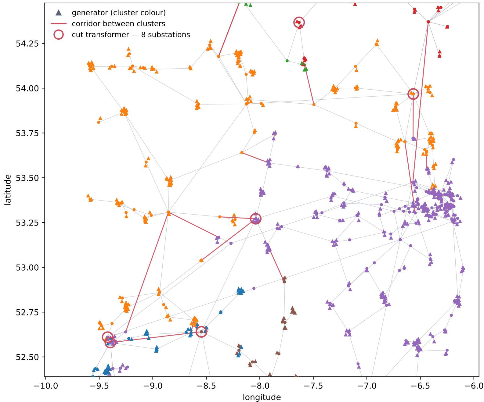
WP2033_all-island +generators — sym, loading, k = 6, 2030-01-20 17:00:00 cluster 1 — 303 nodes
