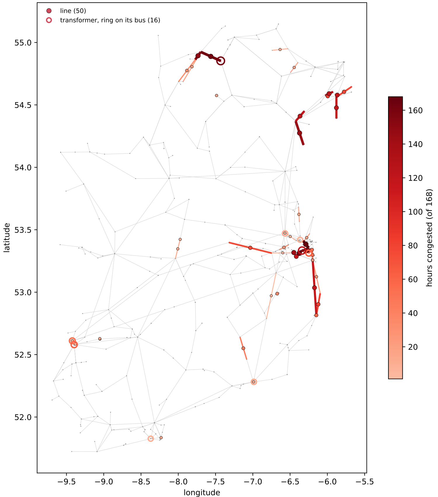
WP2033_all-island (prorata) - branches at \geq 50\% of rating, over 168 hours 66 of 980 branches congested at least once; 0 of them not placeable
