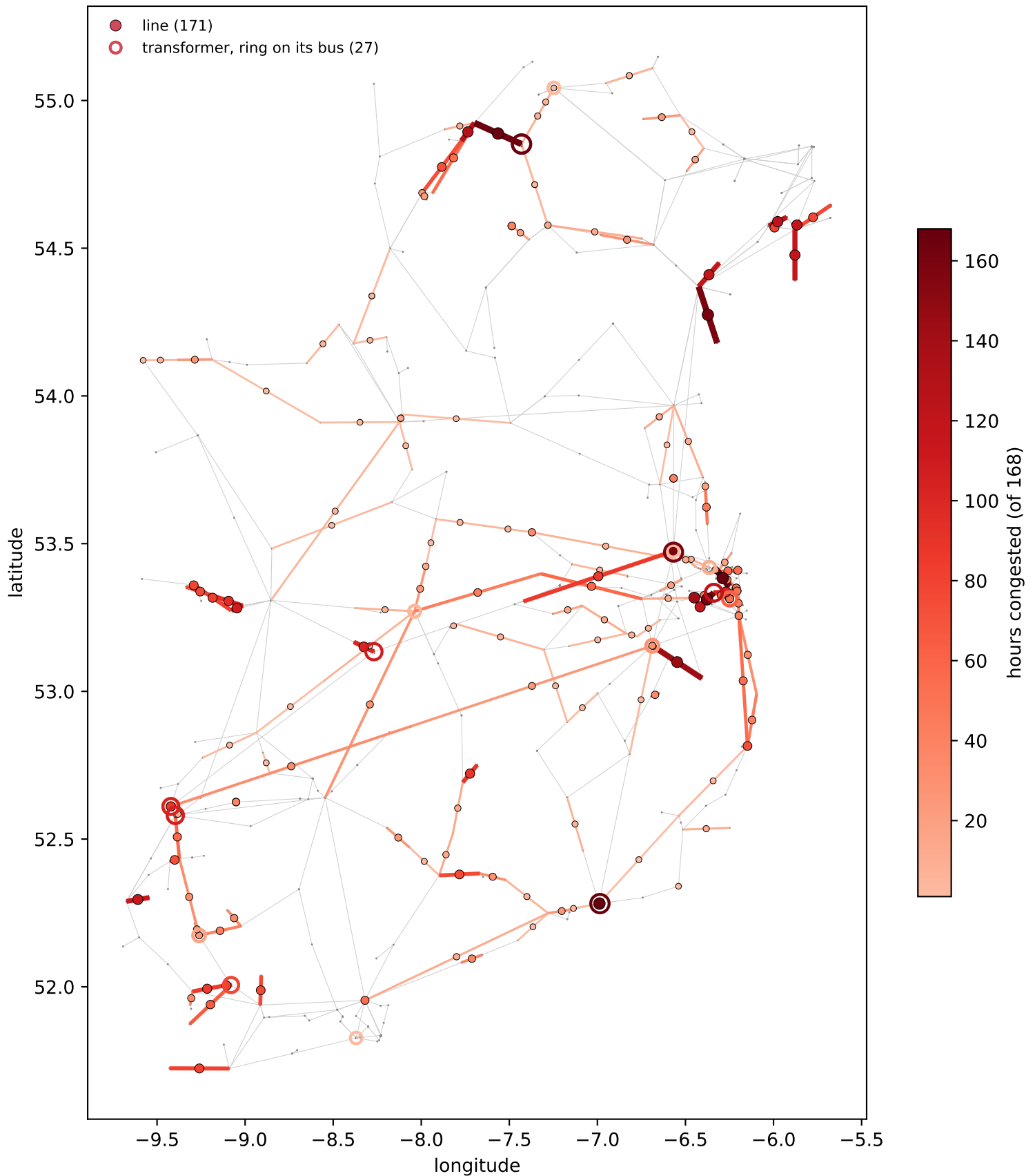
WP2033_all-island (capacity_constrained) - branches at \geq 50\% of rating, over 168 hours 198 of 980 branches congested at least once; 0 of them not placeable
