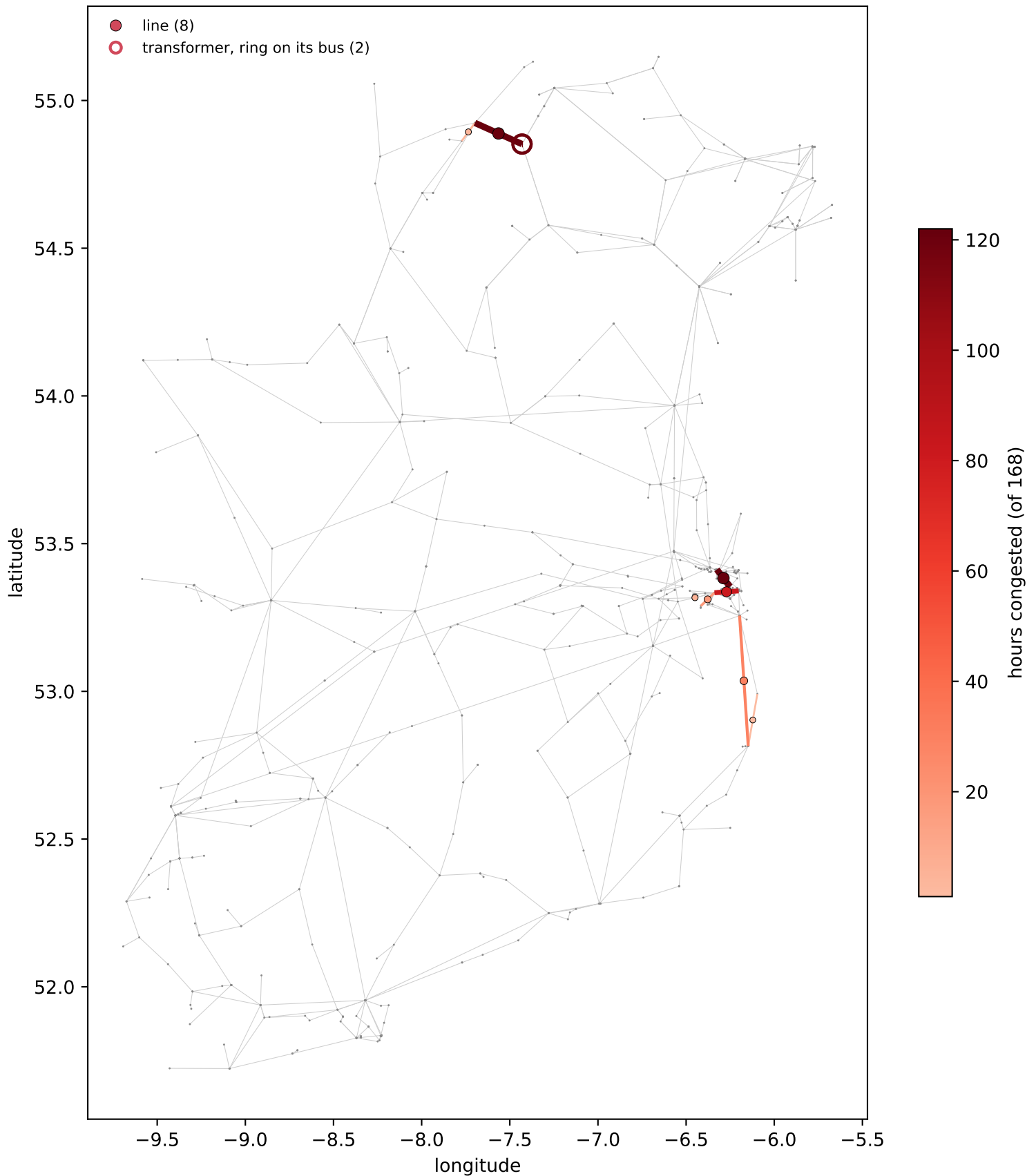
WP2033_all-island (prorata) - branches at \geq 70\% of rating, over 168 hours 10 of 980 branches congested at least once; 0 of them not placeable
