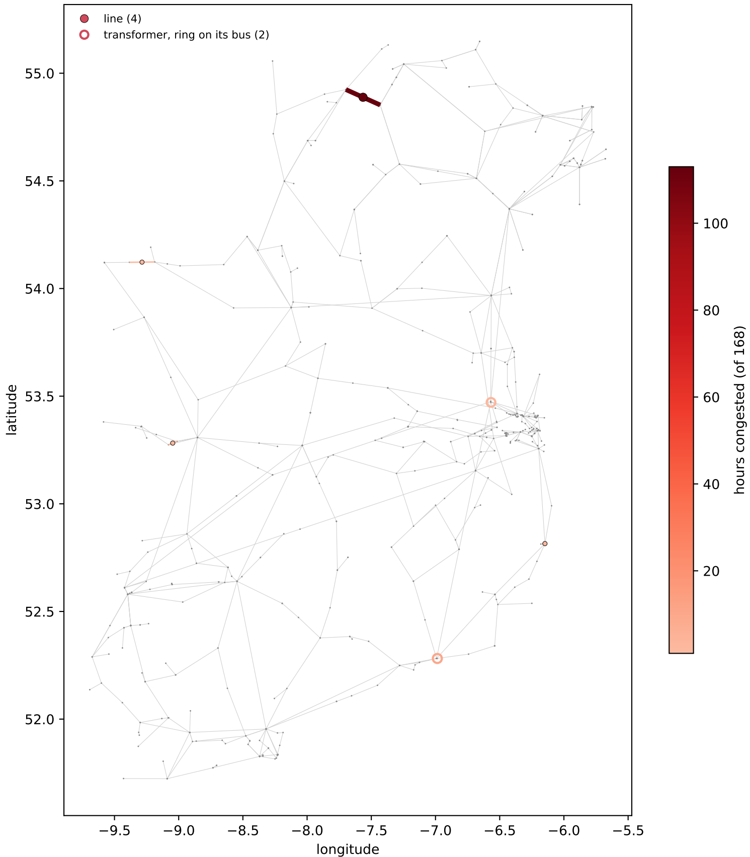
WP2033_all-island (capacity_constrained) - branches at \geq 100\% of rating, over 168 hours 6 of 980 branches congested at least once; 0 of them not placeable
