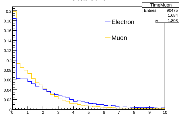
Cluster's time
