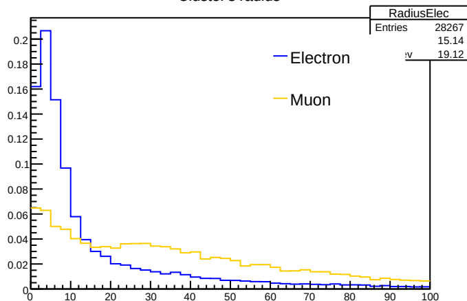
Cluster's radius
