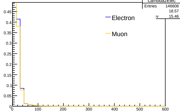
Cluster's lambda2
