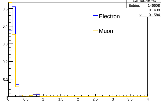
Cluster's lambda
