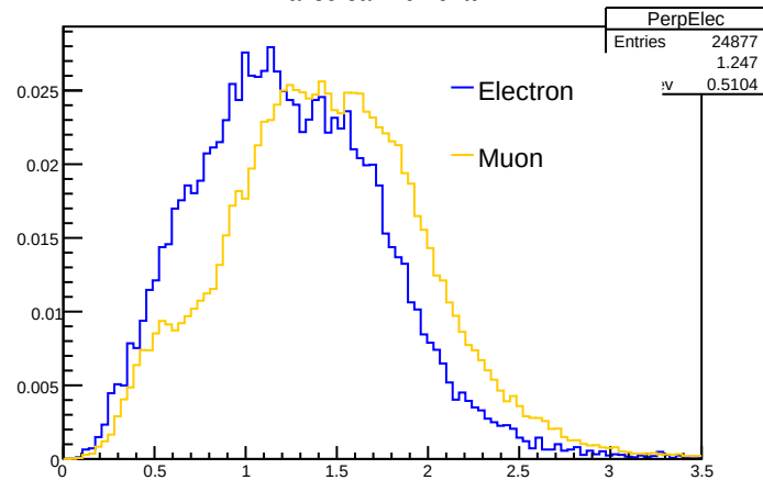
Traversal momentum
