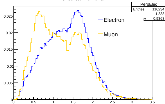
Transversal momentum
