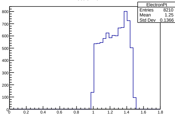
ElectronPt
