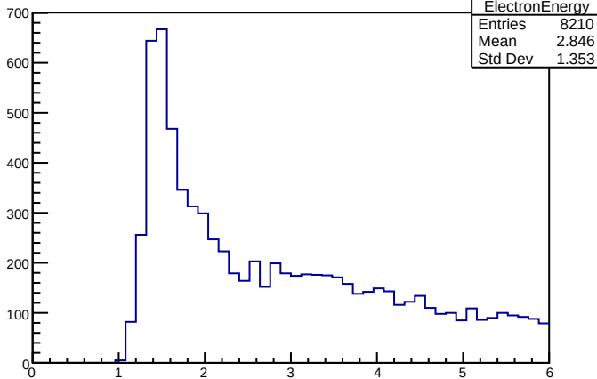
ElectronEnergy
