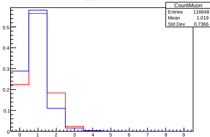
CountMuon
