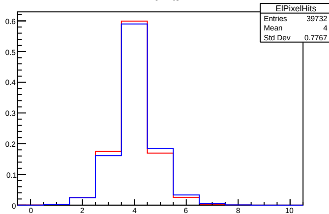
PixelHits
