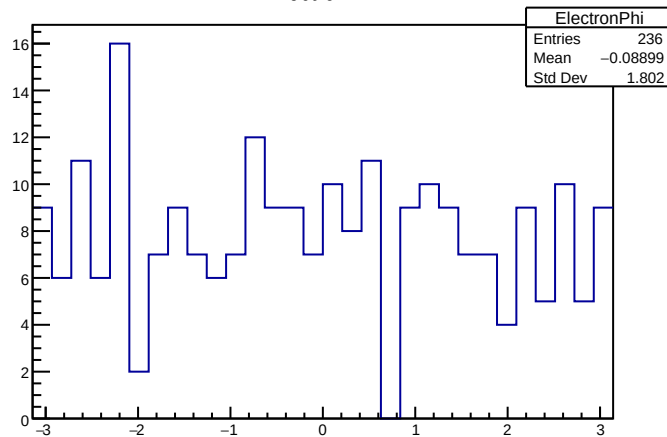
ElectronPhi
