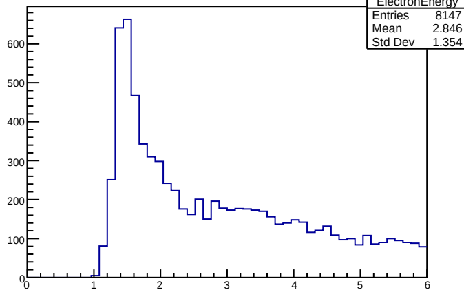
ElectronEnergy
