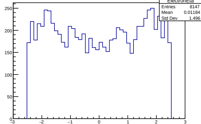
ElectronEta
