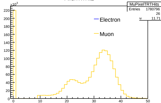
PixelTRTHits
