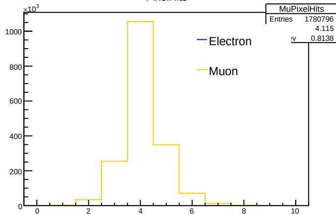
PixelHits
