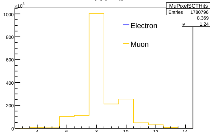
PixelSCTHits
