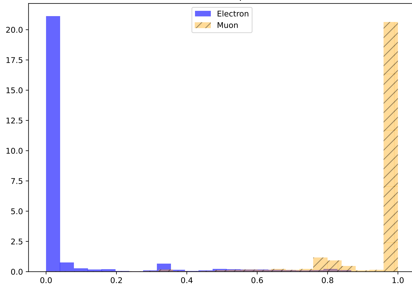
Classifier Response
