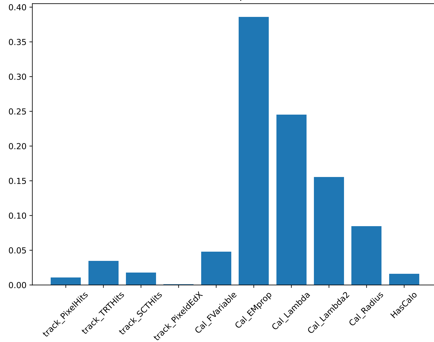
Feature Importance
