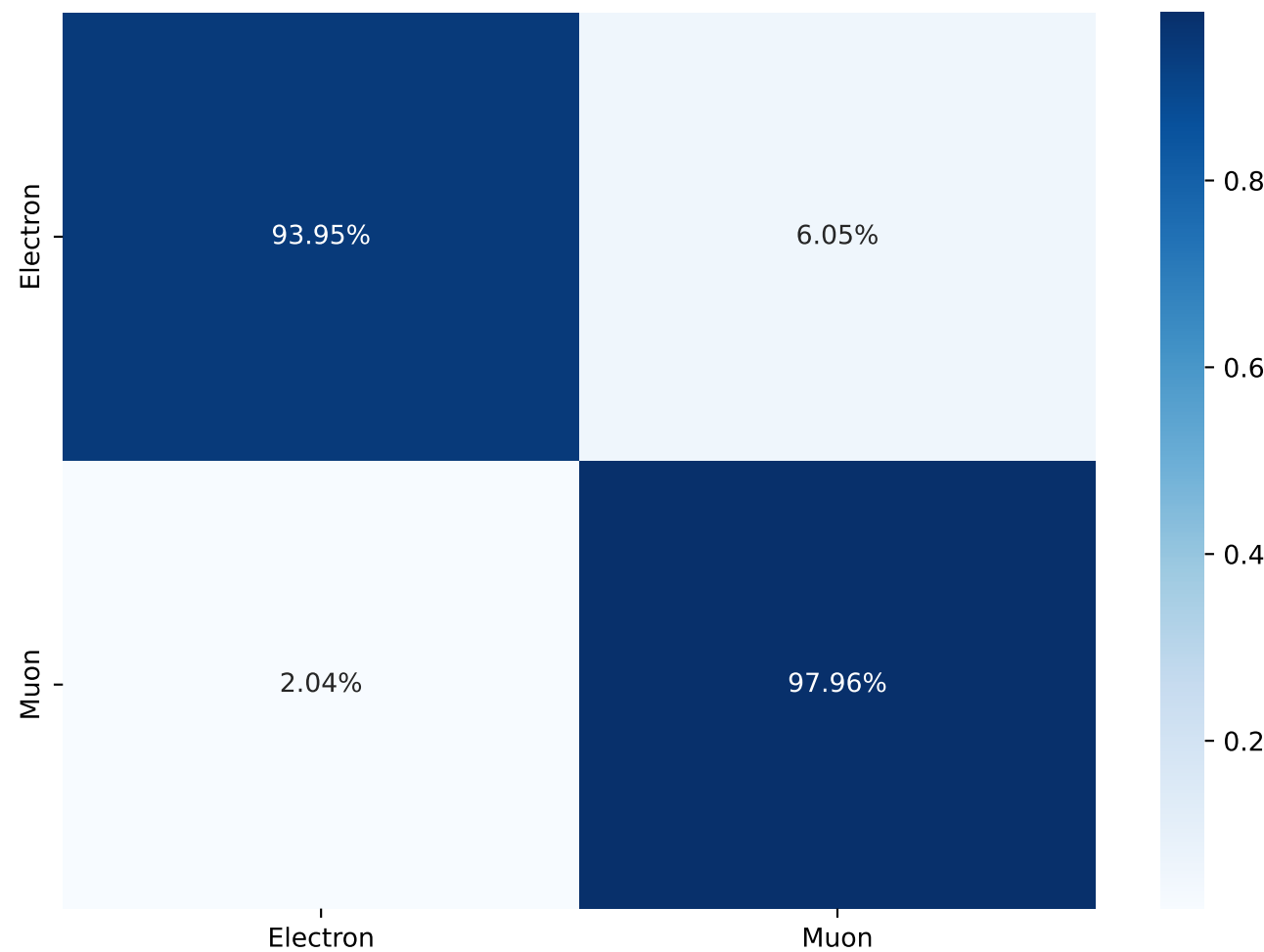
Classifier Response
