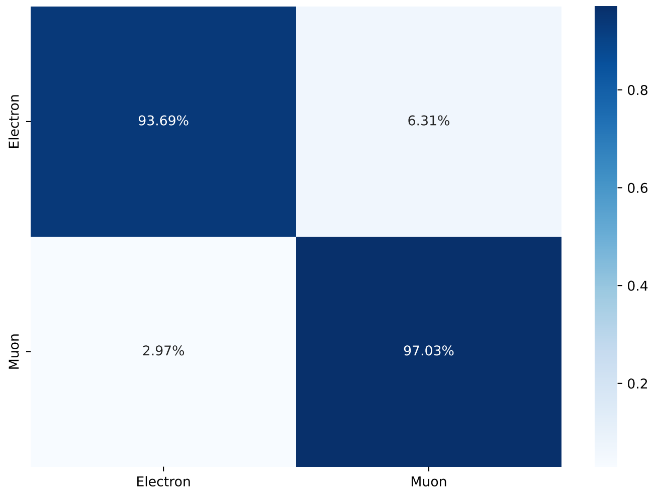
Classifier Response
