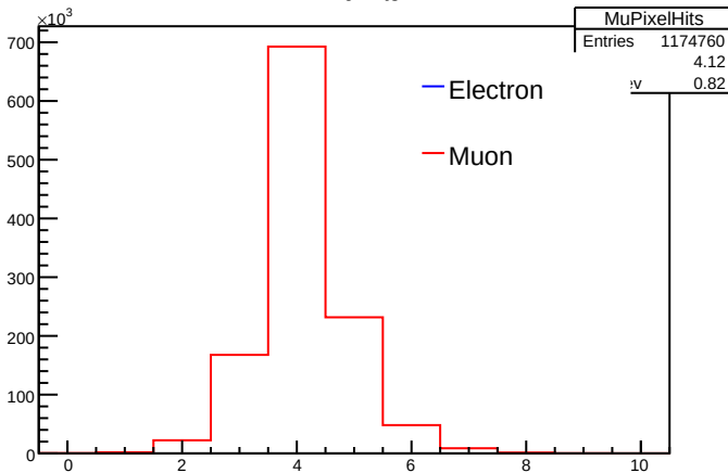
PixelHits
