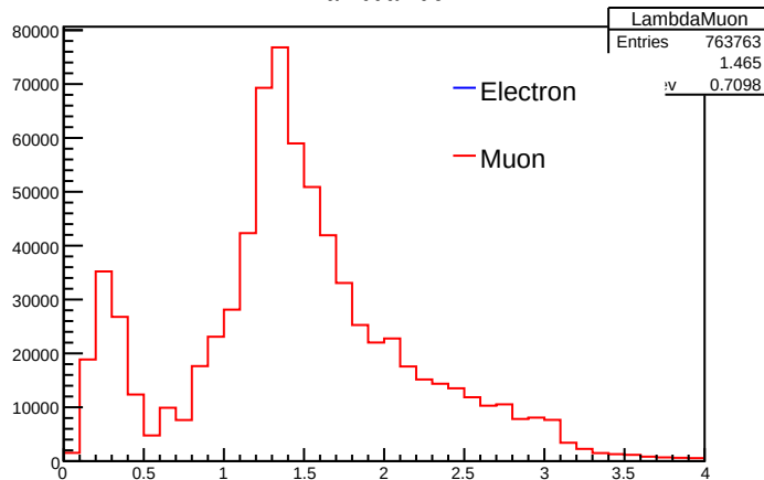
LambdaMuon
