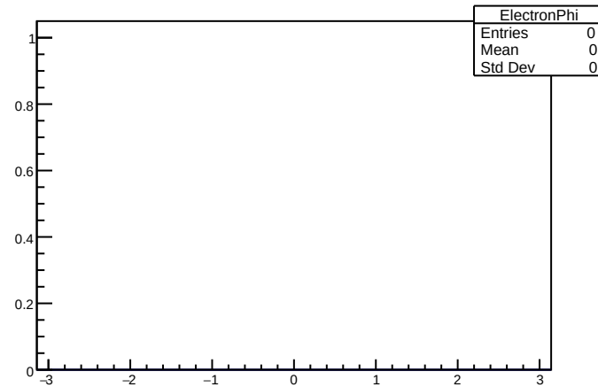
ElectronPhi
