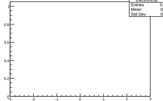
ElectronEta
