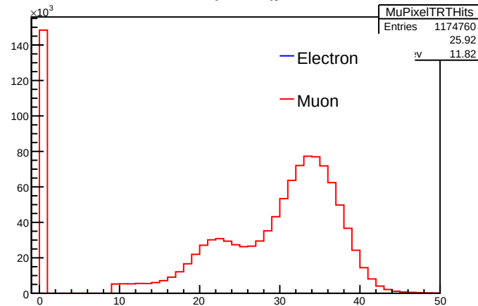
PixelTRTHits
