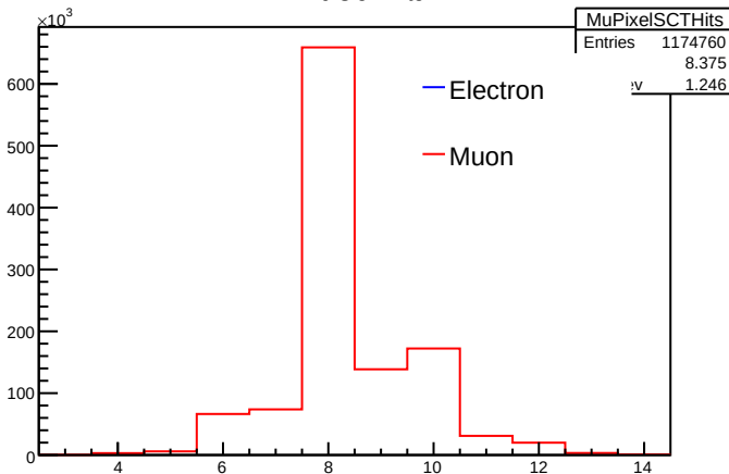
PixelSCTHits
