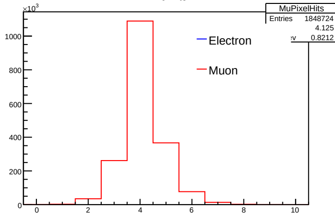
PixelHits
