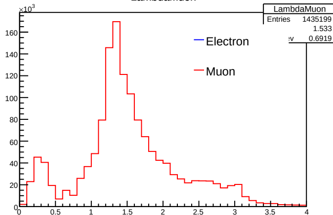
LambdaMuon
