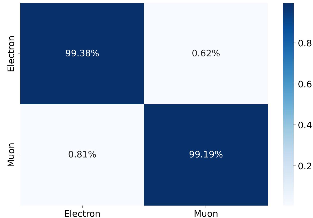
Confusion Matrix
