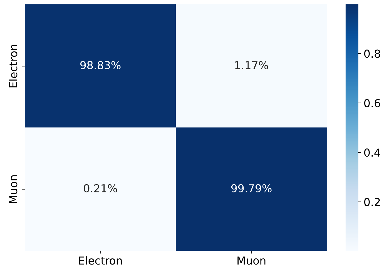
Classifier Response
