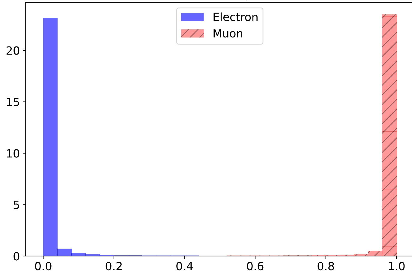
Classifier Response
