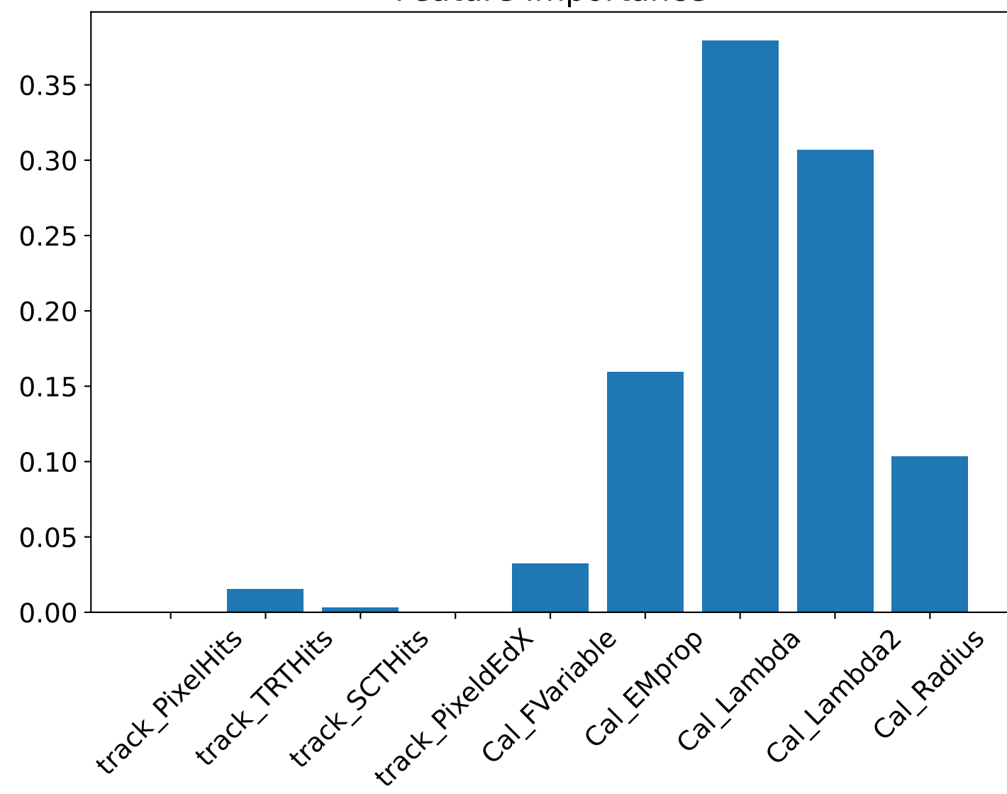
Feature Importance
