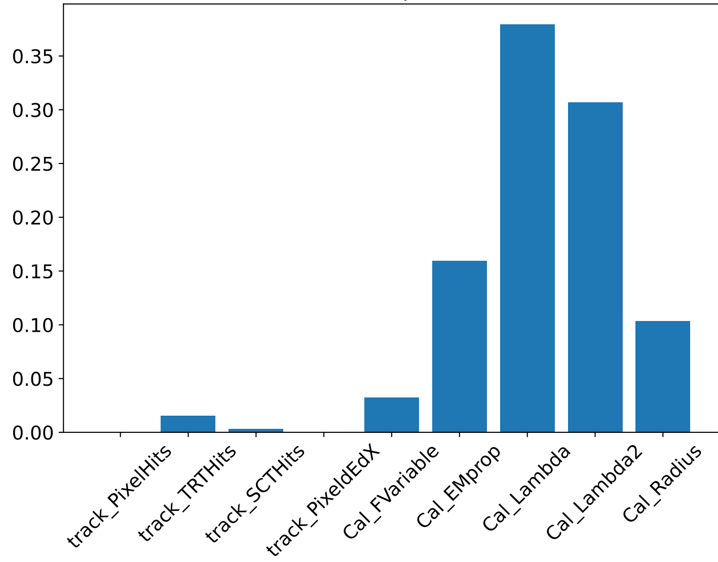
Feature Importance
