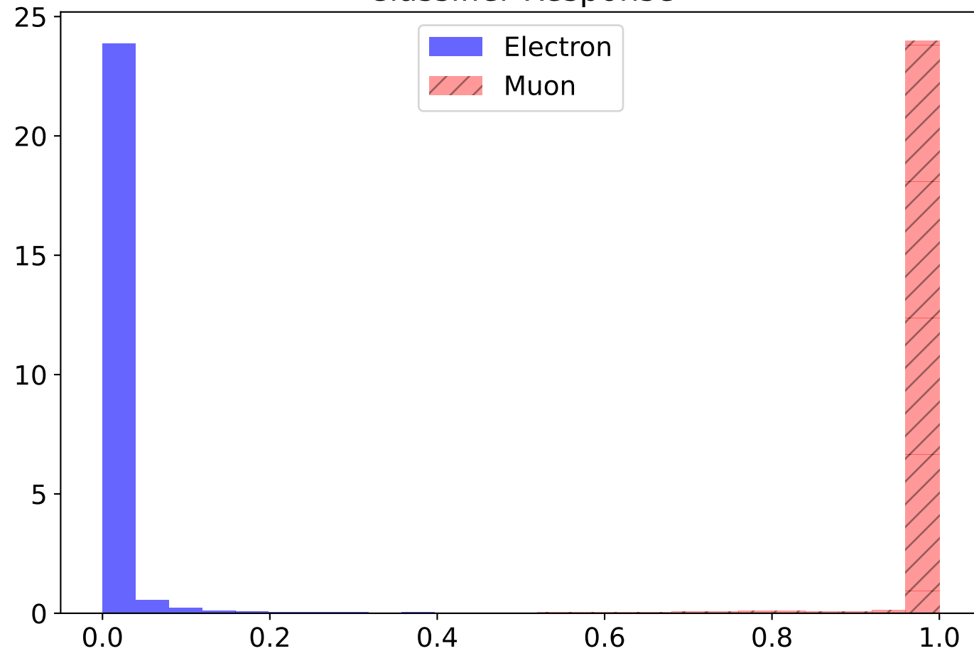
Classifier Response
