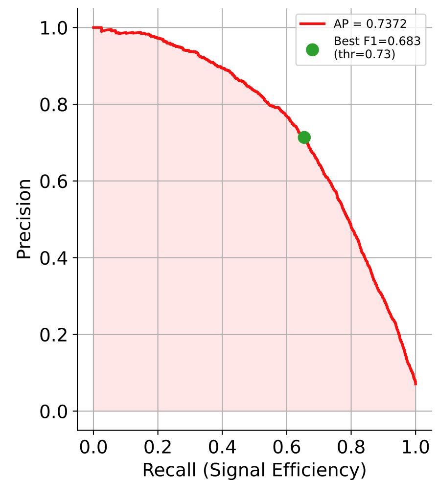
Precision-Recall Curve
