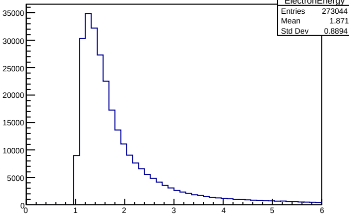
ElectronEnergy
