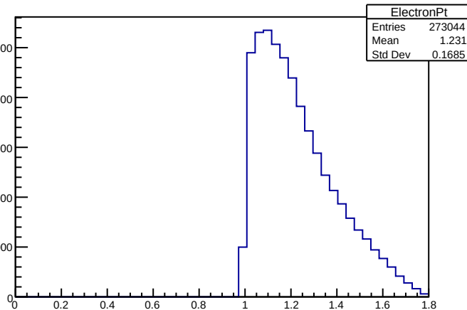
ElectronPt
