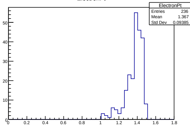
ElectronPt
