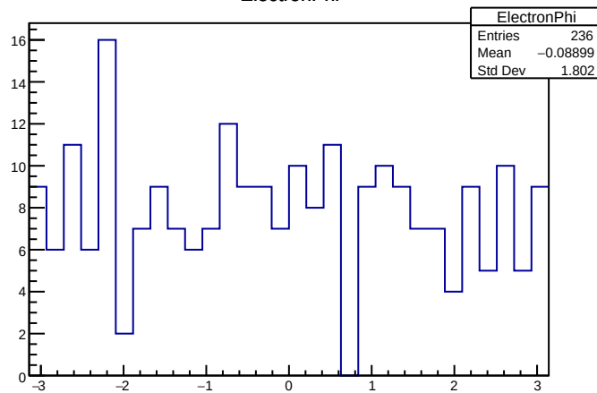
ElectronPhi
