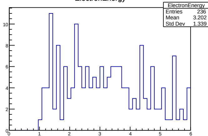
ElectronEnergy
