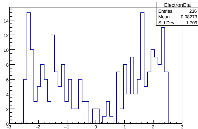
ElectronEta
