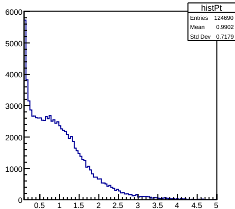
histPt
