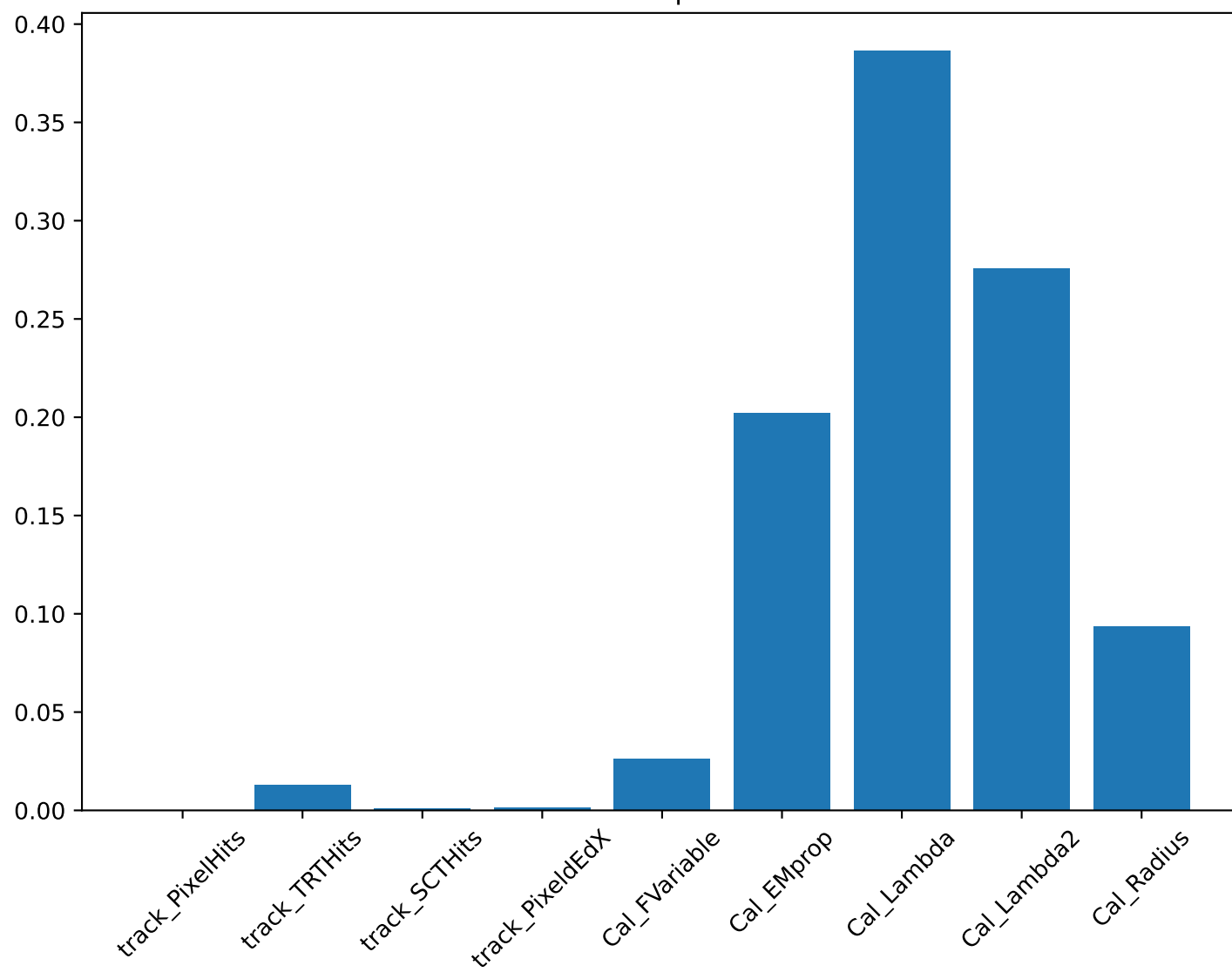
Feature Importance
