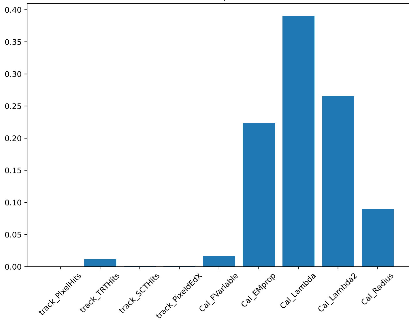
Feature Importance
