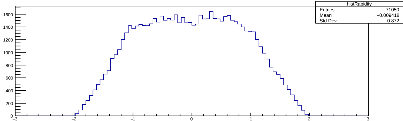
histRapidity
