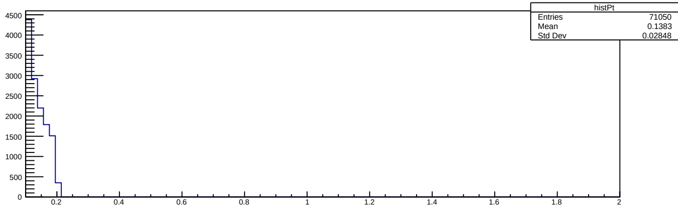
histPt
