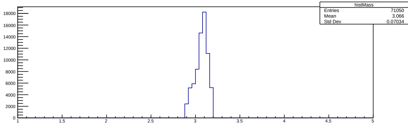
histMass
