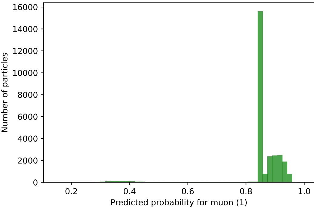
Predicted probabilities
