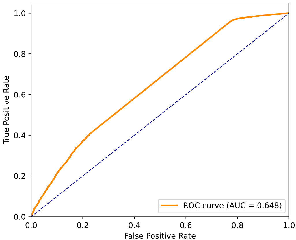
ROC Curve
