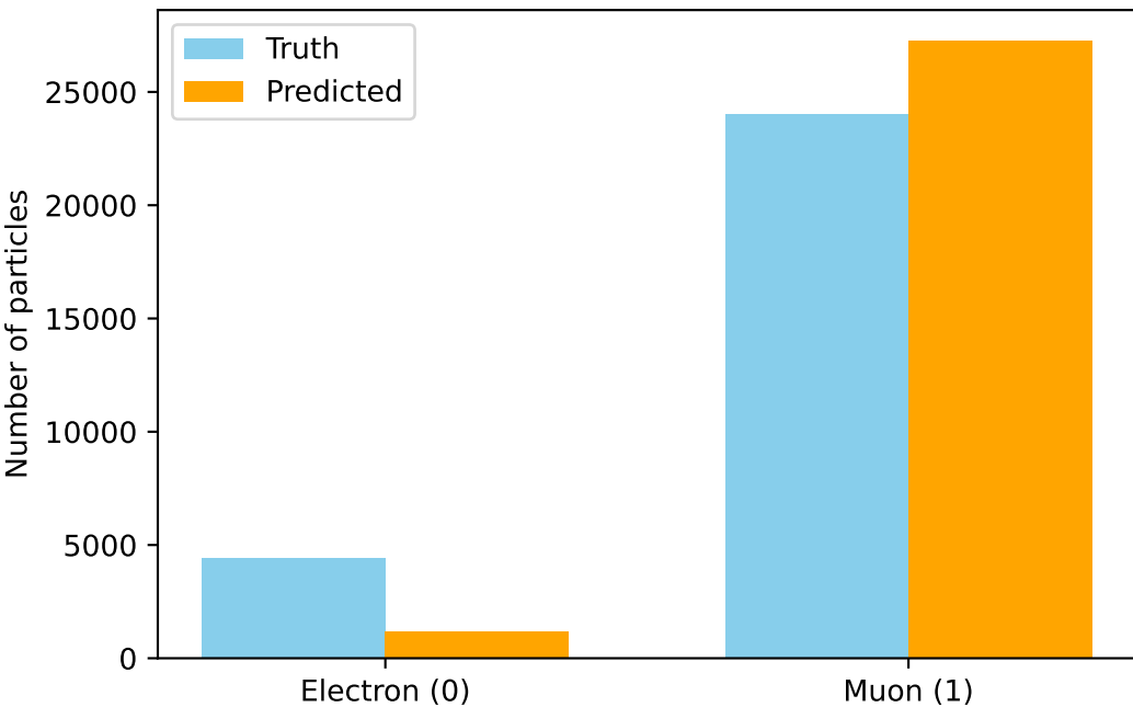
Predicted vs Truth particles
