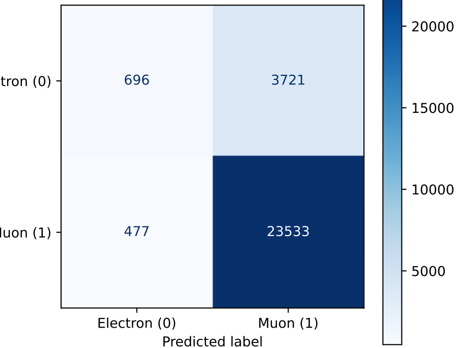
Confusion Matrix
