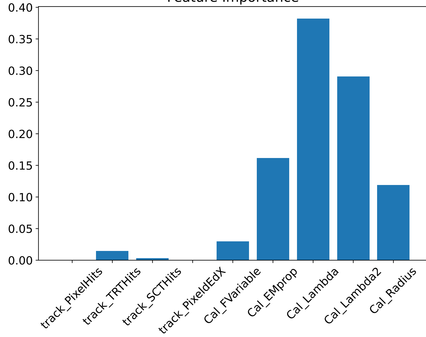
Feature Importance
