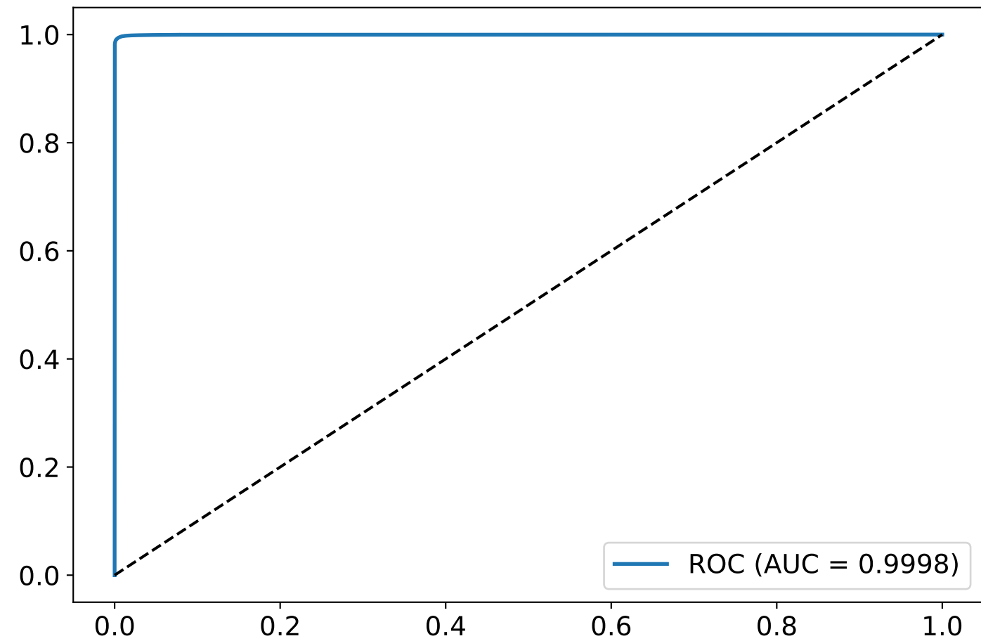
ROC Curve
