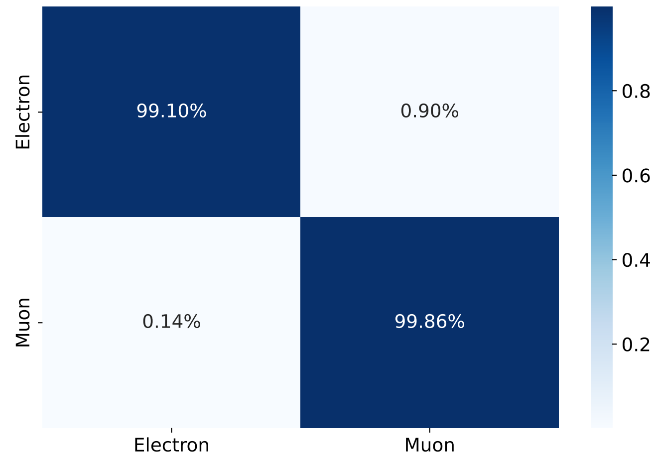
Classifier Response
