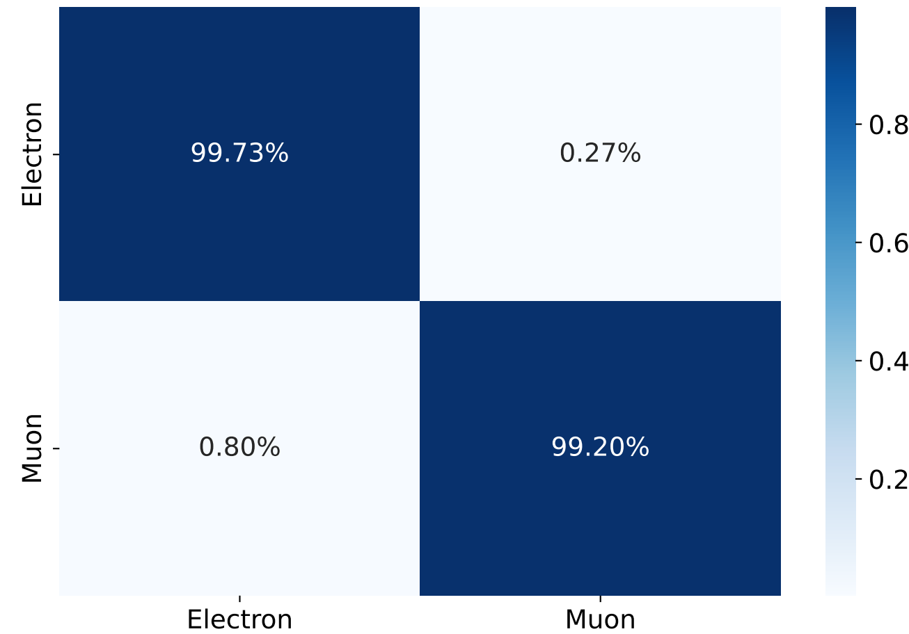
Confusion Matrix
