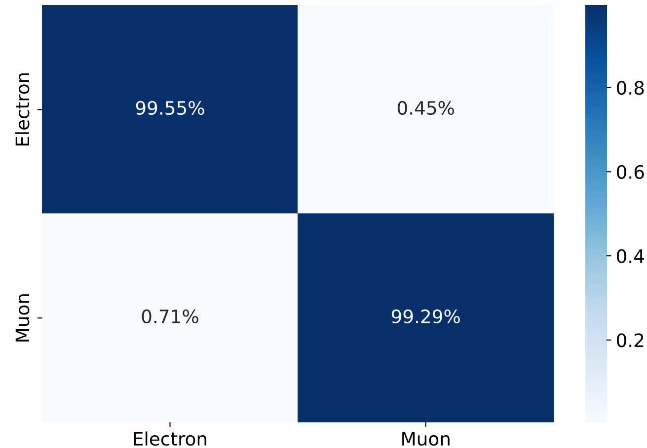
Confusion Matrix
