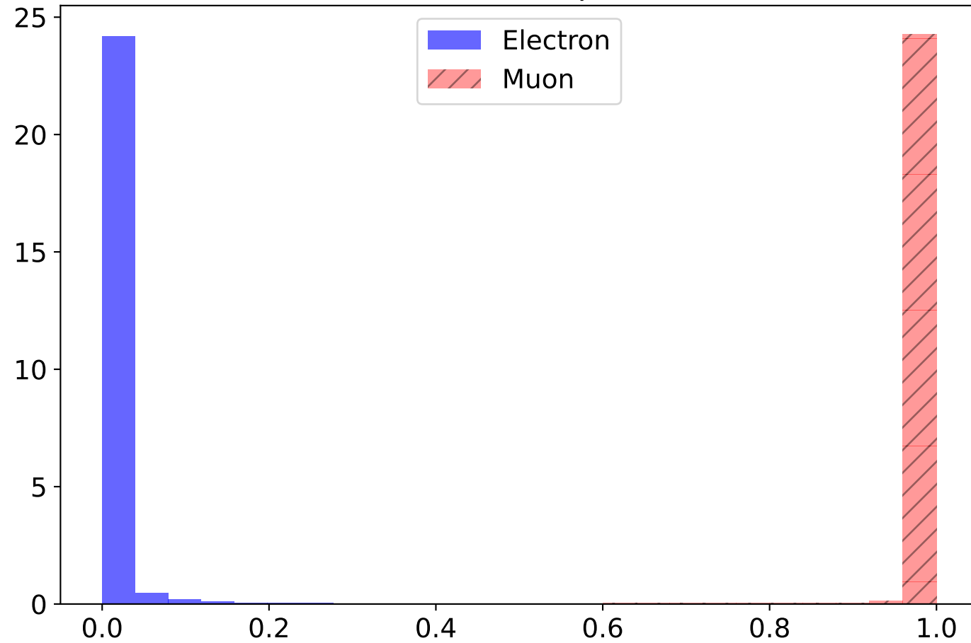
Classifier Response
