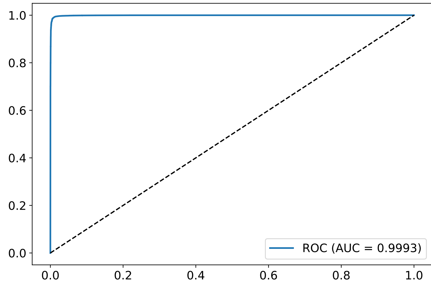
ROC Curve
