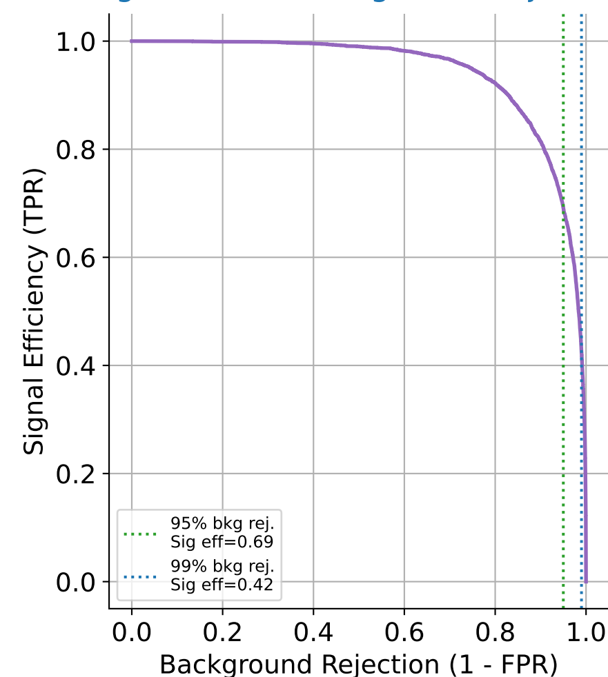
Signal Eff. vs Background Rejection
