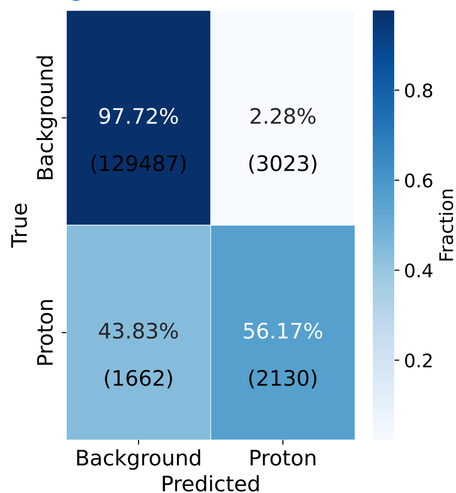
Confusion Matrix @ Max F1-Score (thr=0.86)
