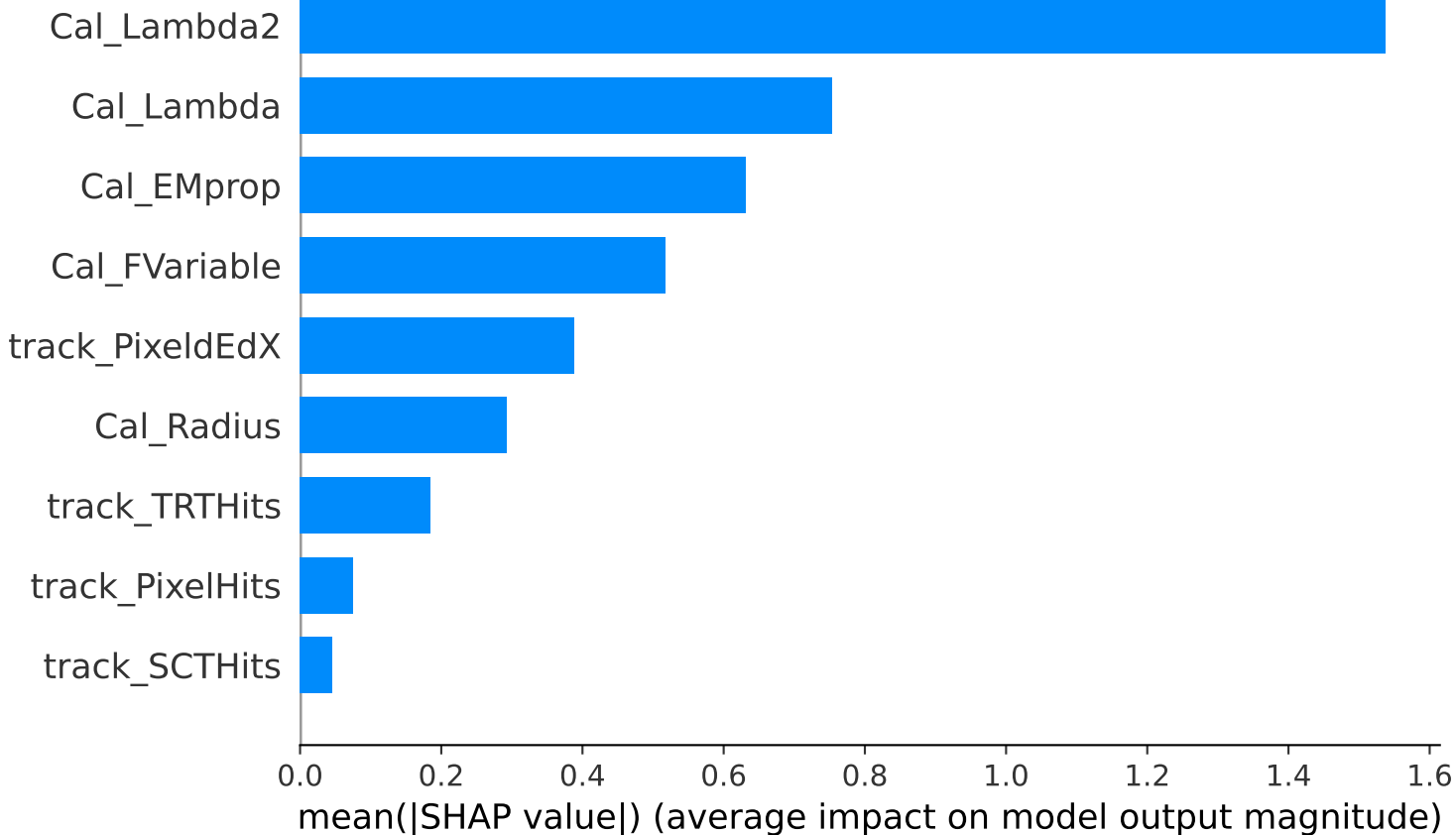
SHAP Feature Importance (mean |SHAP|)
