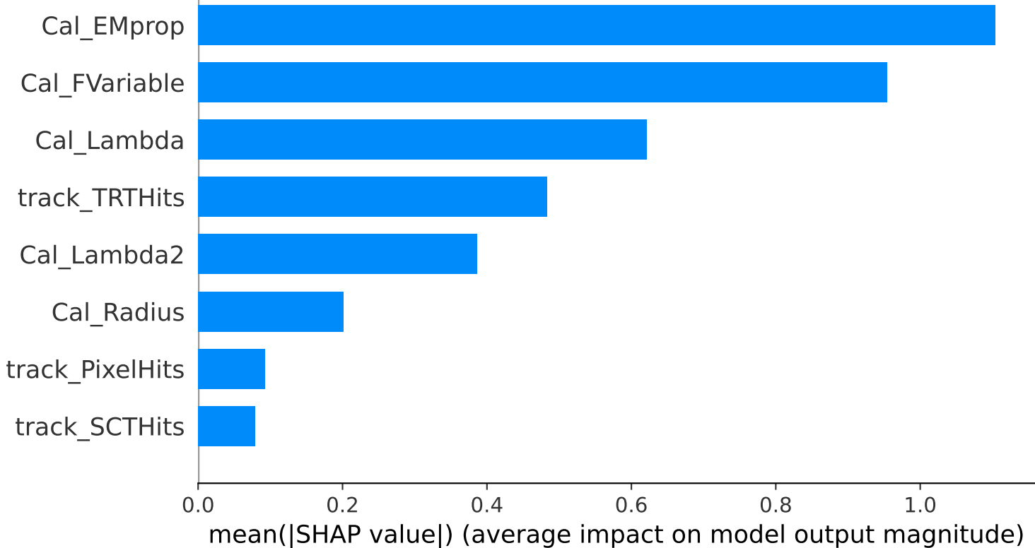
SHAP Feature Importance (mean |SHAP|)
