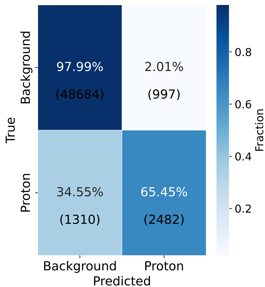
Confusion Matrix @ Max F1-Score (thr=49897)
