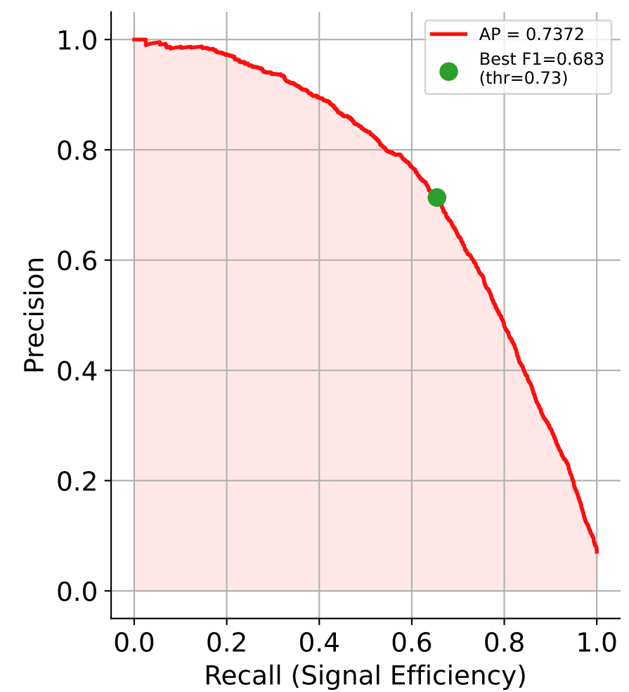
Precision-Recall Curve
