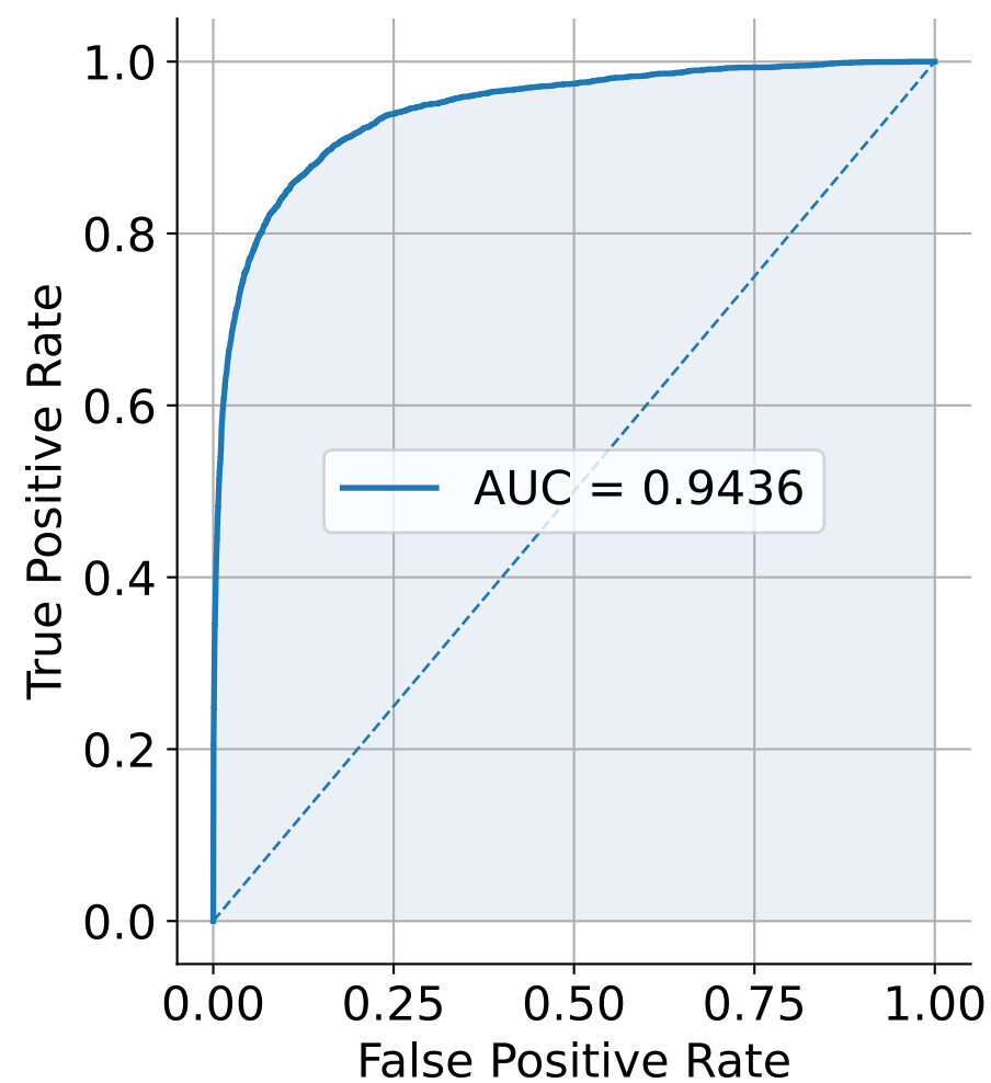
ROC Curve
