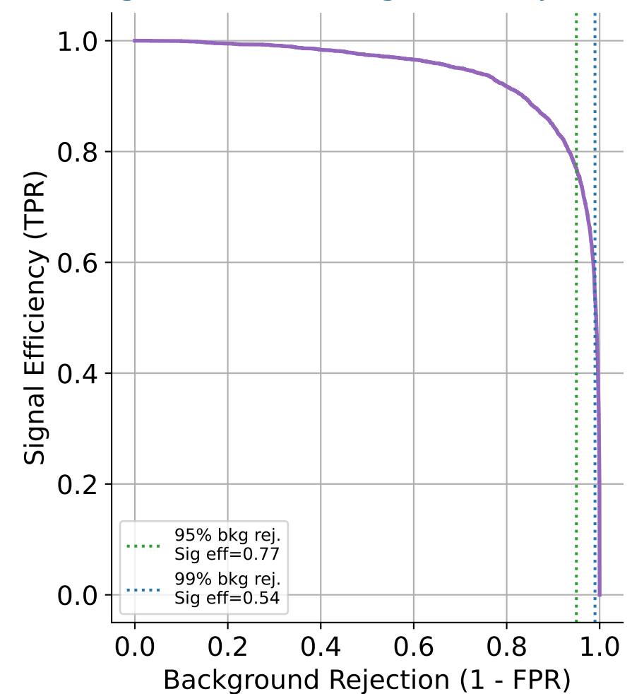
Signal Eff. vs Background Rejection
