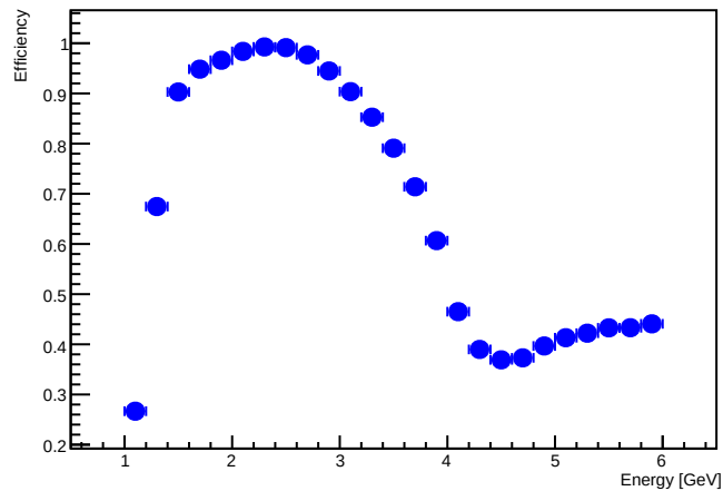
Calorimetr Found efficiency - MCμμ
