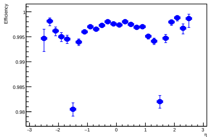
Algorithm Efficiency - MC ee
