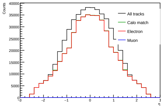
\eta distributions - MC ee
