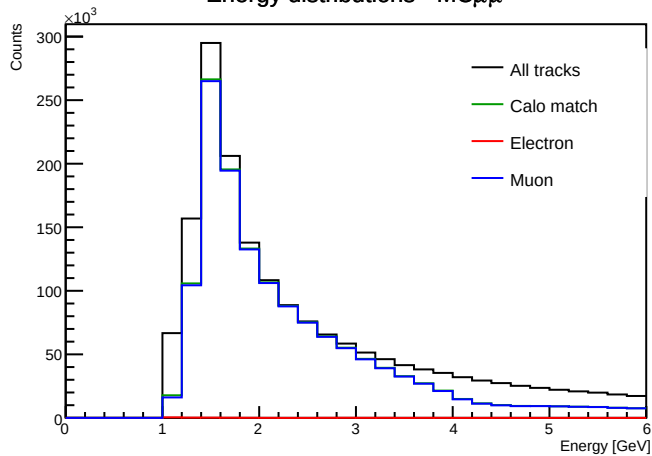
Energy distributions - MCμμ
