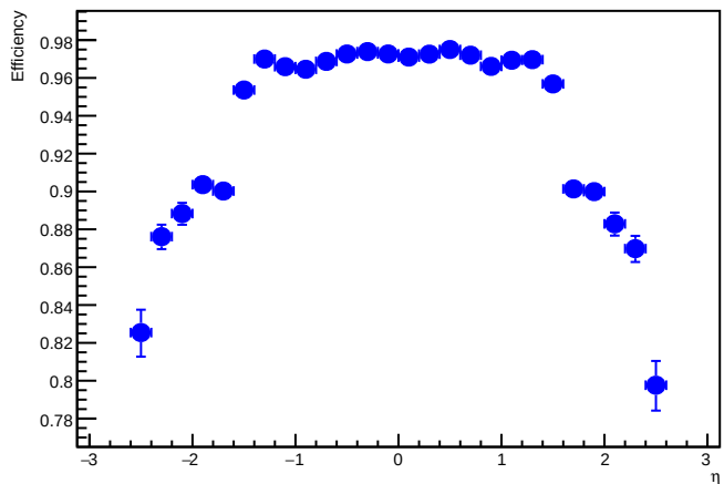
Algorithm Efficiency - Data
