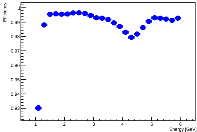
Algorithm Found efficiency - MCμμ
