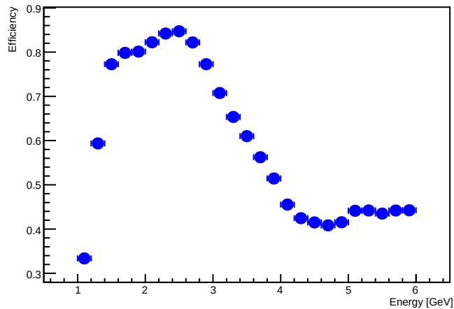
Calorimetr Found efficiency - Data
