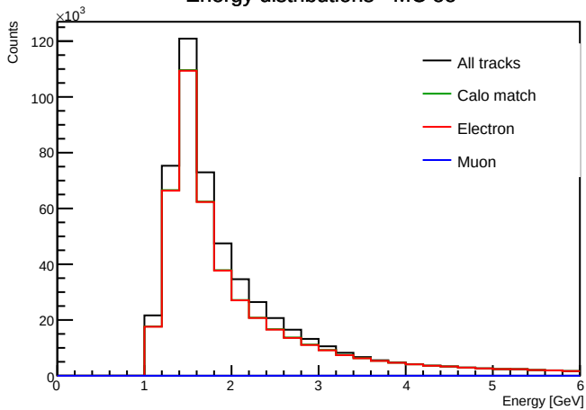
Energy distributions - MC ee
