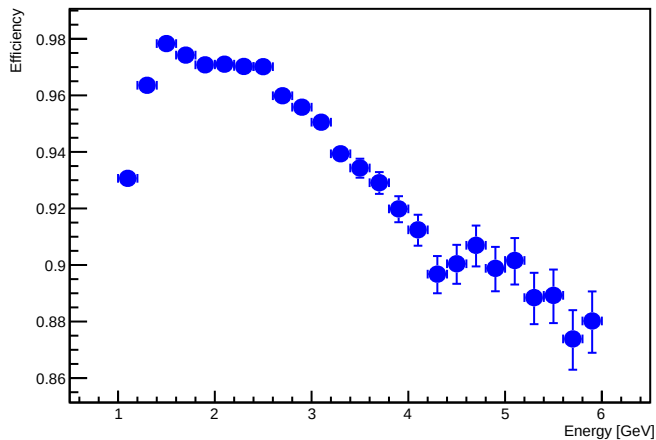
Algorithm Found efficiency - Data
