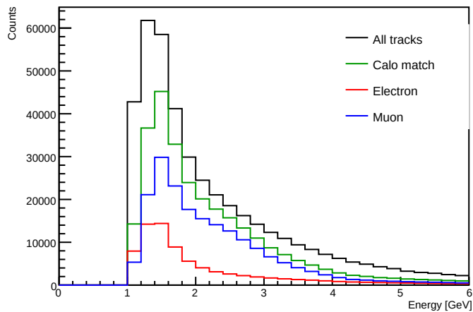
Energy distributions - Data
