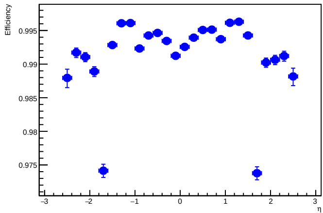
Algorithm Efficiency - MC \mu\mu
