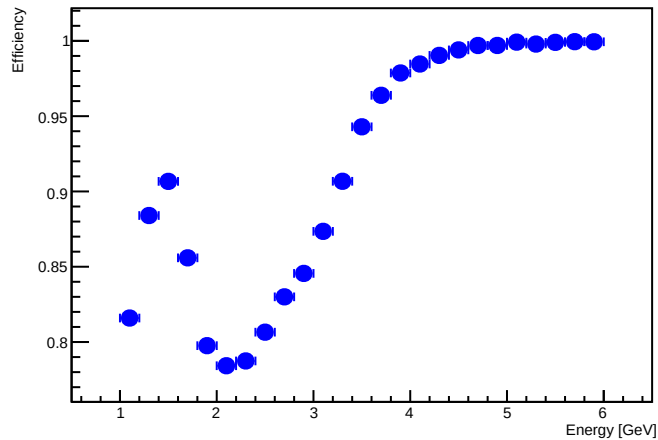
Calorimetr Found efficiency - MC ee
