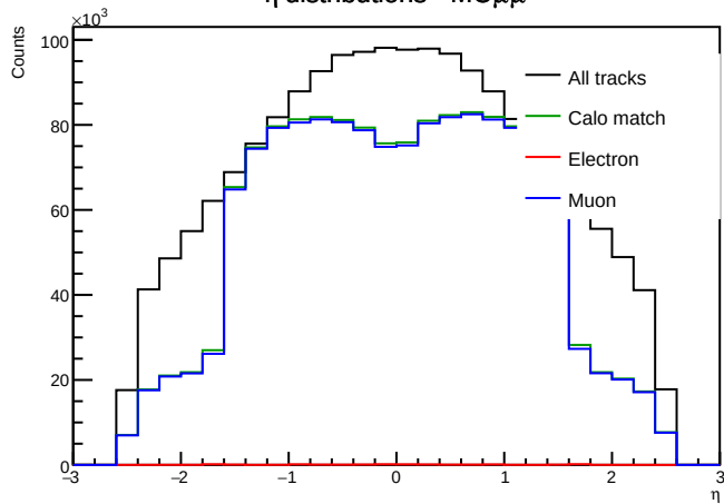
\eta distributions - MC \mu\mu
