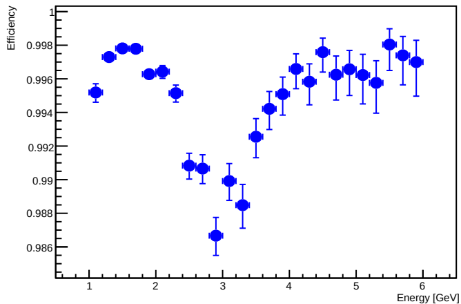
Algorithm Found efficiency - MC ee
