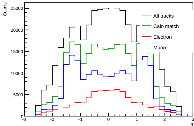
\eta distributions - Data
