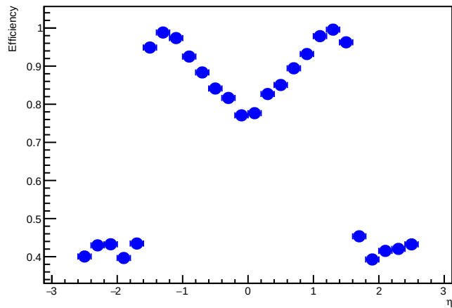
Topocluster Reconstruction Efficiency - MC \mu\mu
