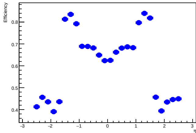
Topocluster Reconstruction Efficiency - Data
