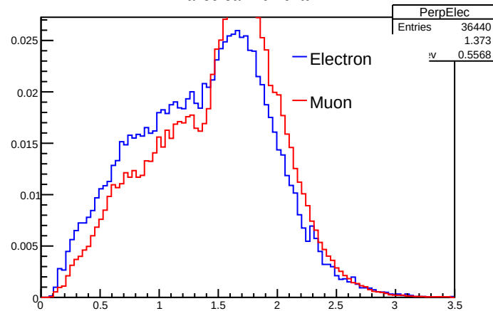
Traversalal momentum
