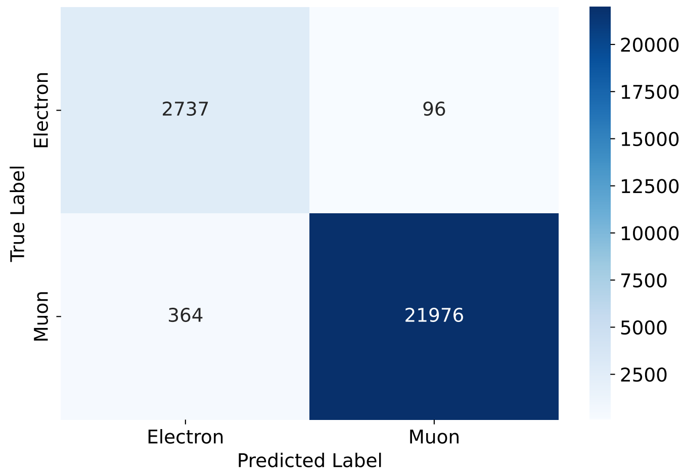
Classifier Response (MC)
