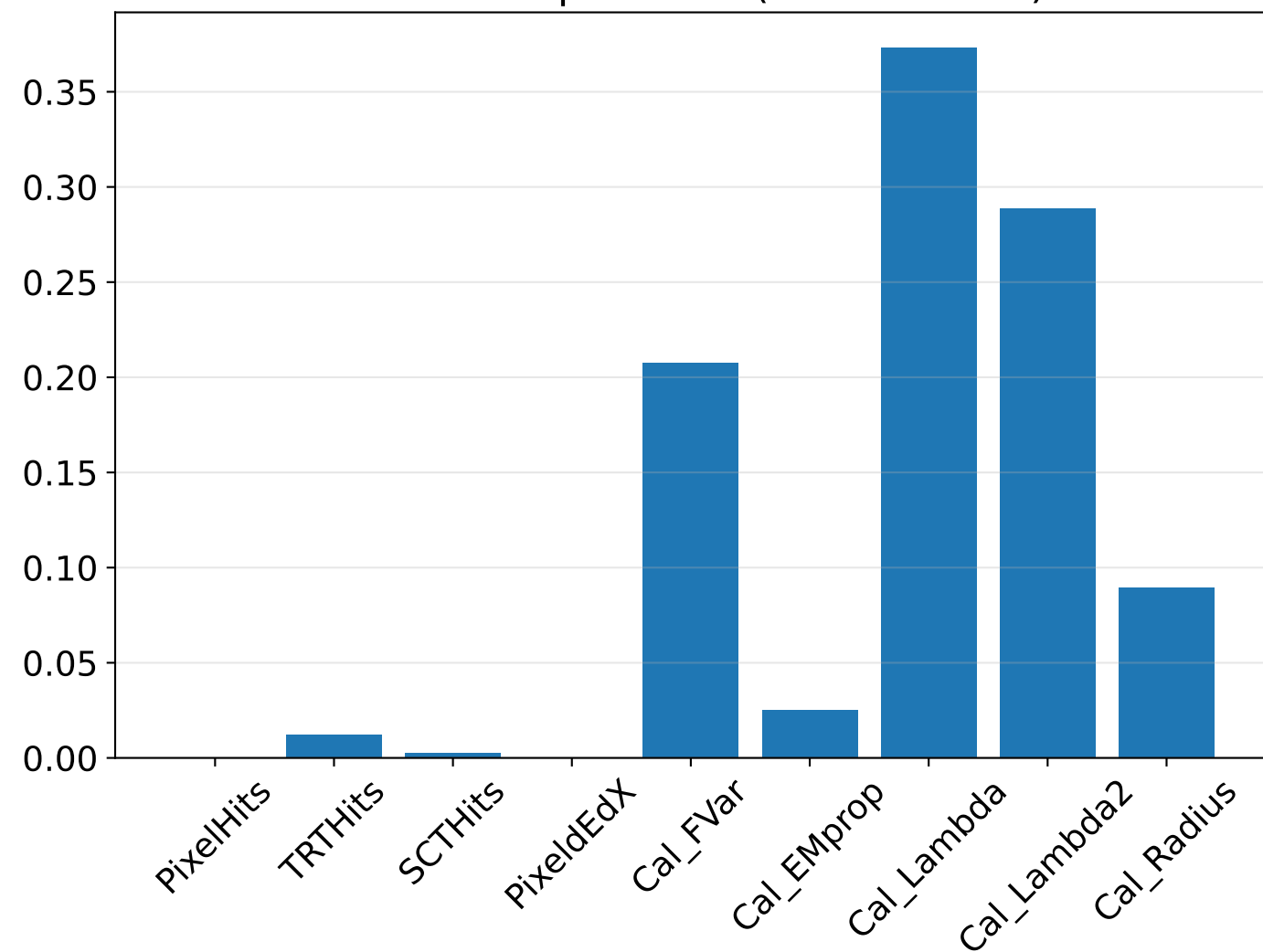
Feature Importance (full TrueData)
