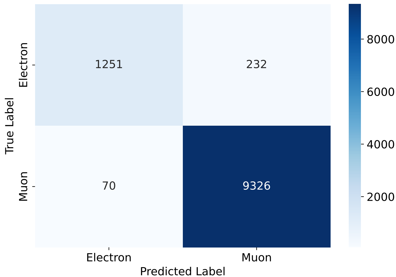
Confusion Matrix
