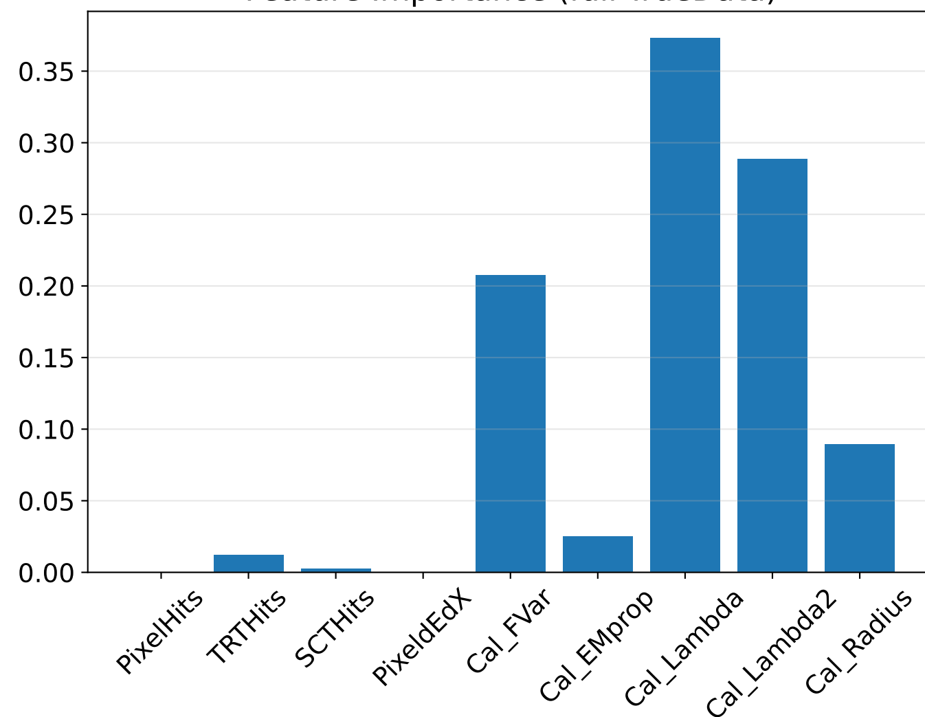
Feature Importance (full TrueData)
