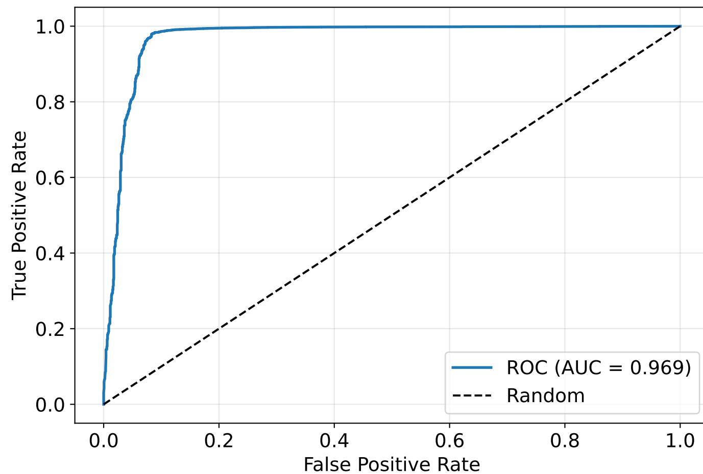
ROC Curve
