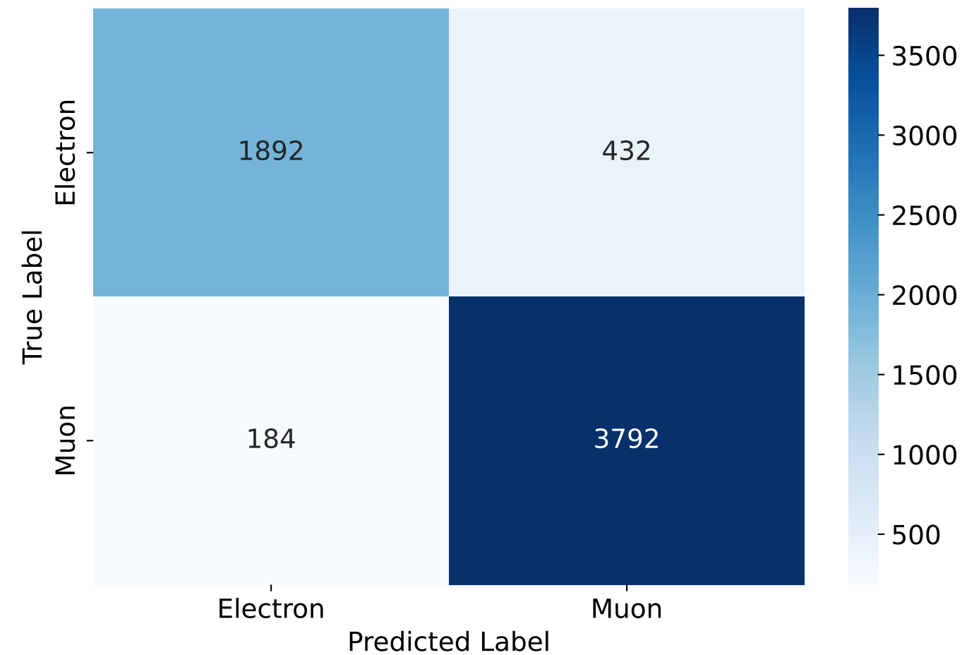
Confusion Matrix
