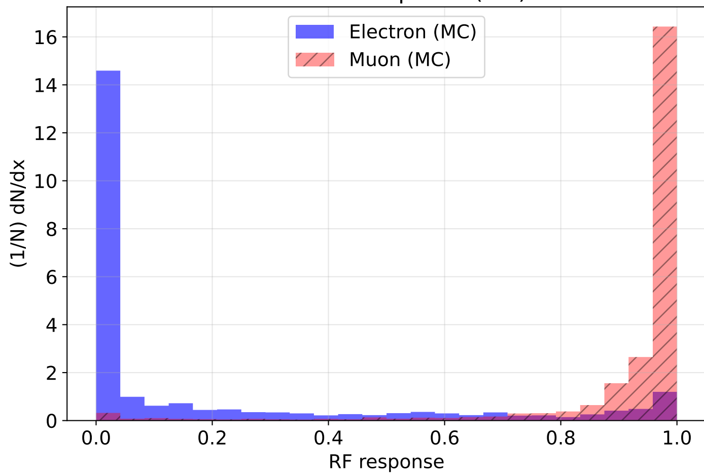
Classifier Response (MC)
