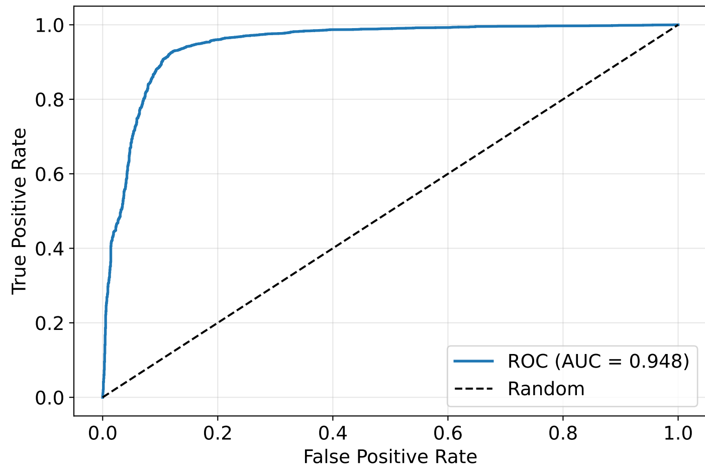
ROC Curve
