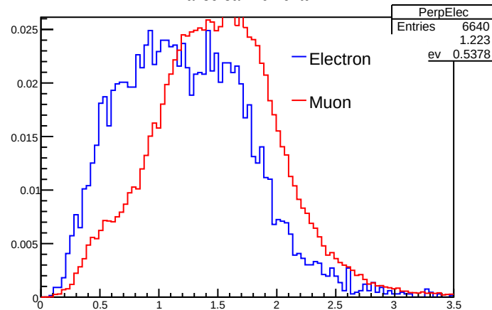
Traversal momentum
