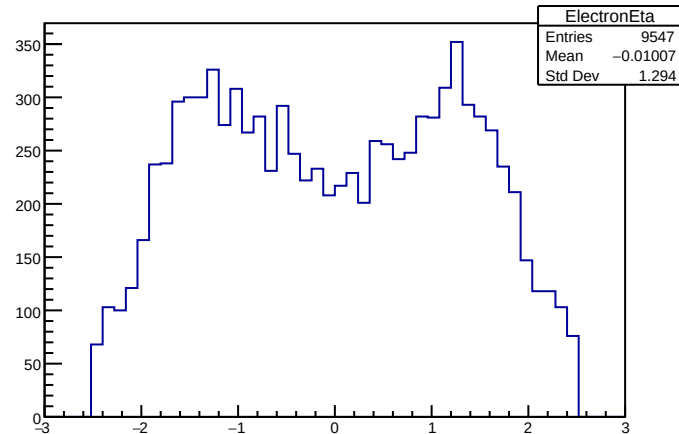
ElectronEta
