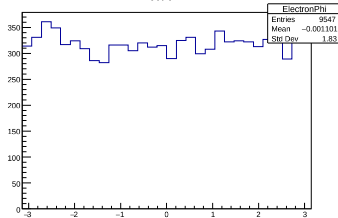
ElectronPhi
