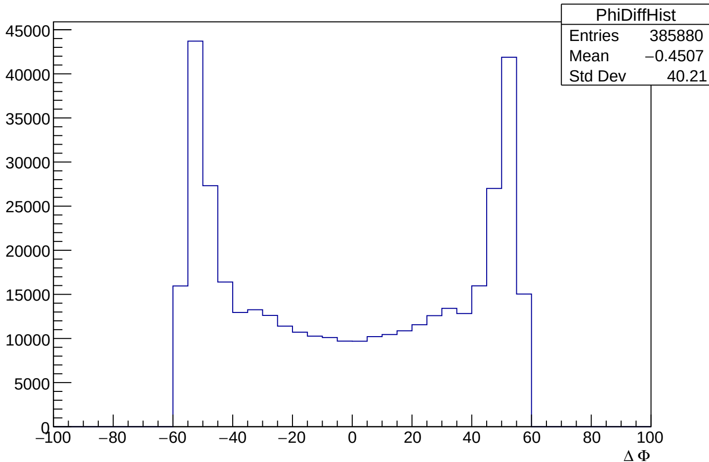
PhiDiffHist
