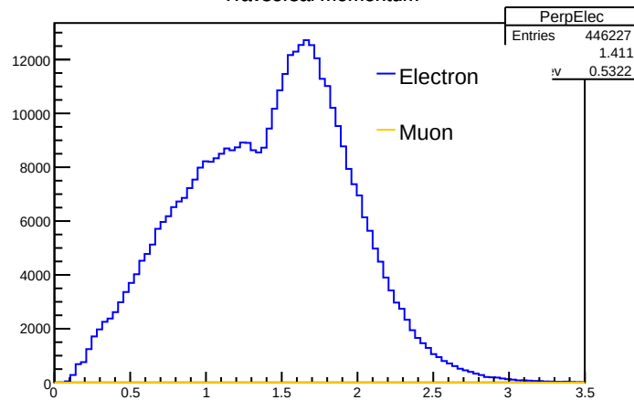
Transversal momentum
