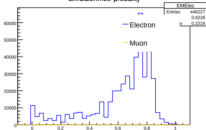
EMCalorimetr probablity
