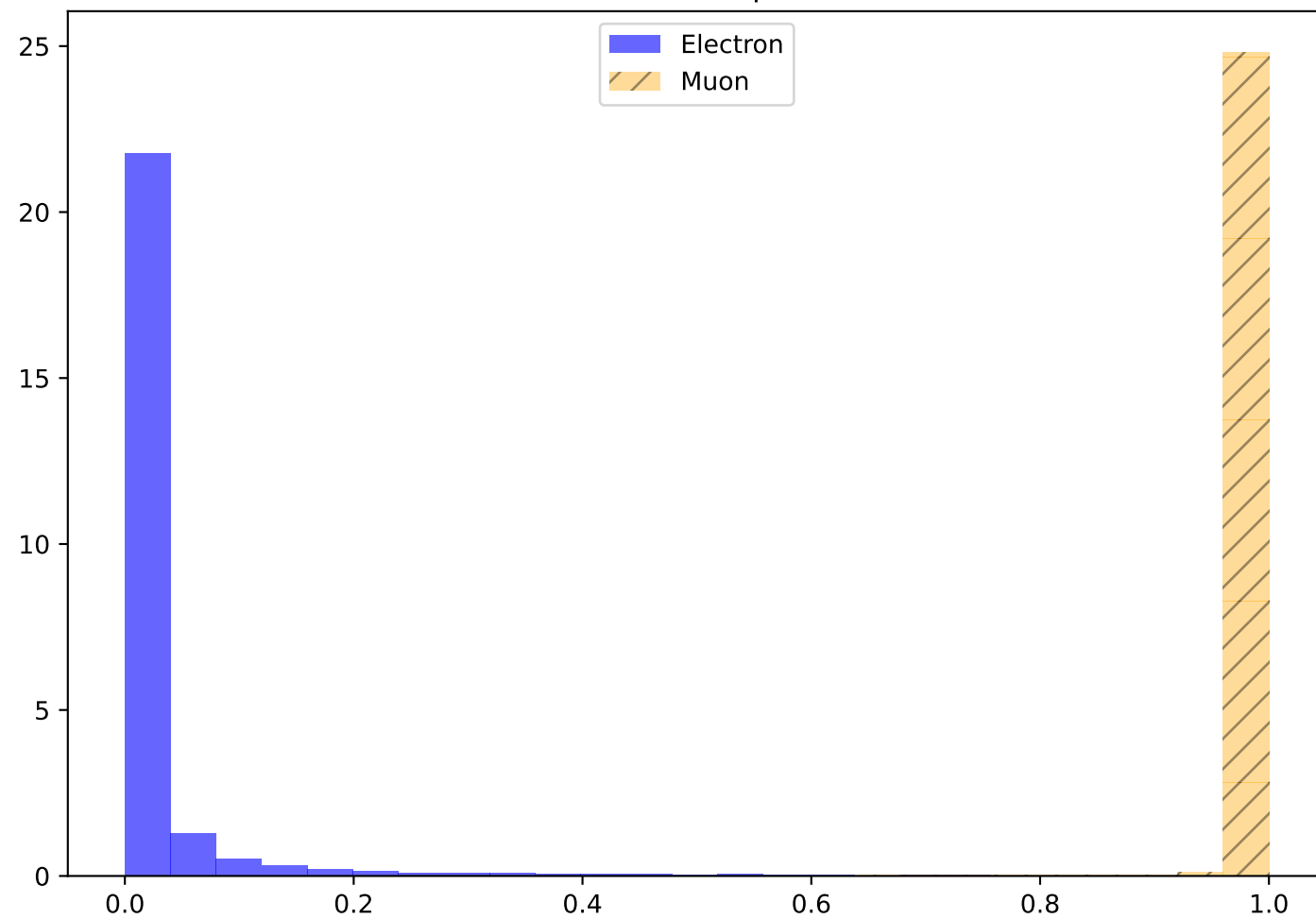
Classifier Response
