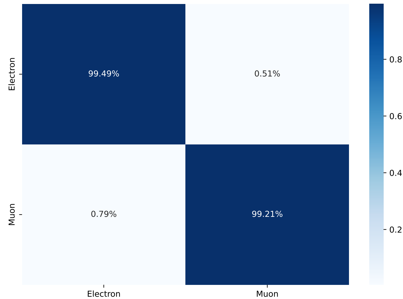
Classifier Response
