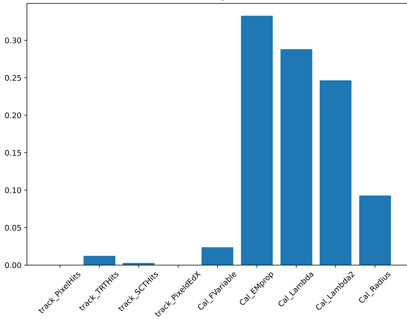
Feature Importance
