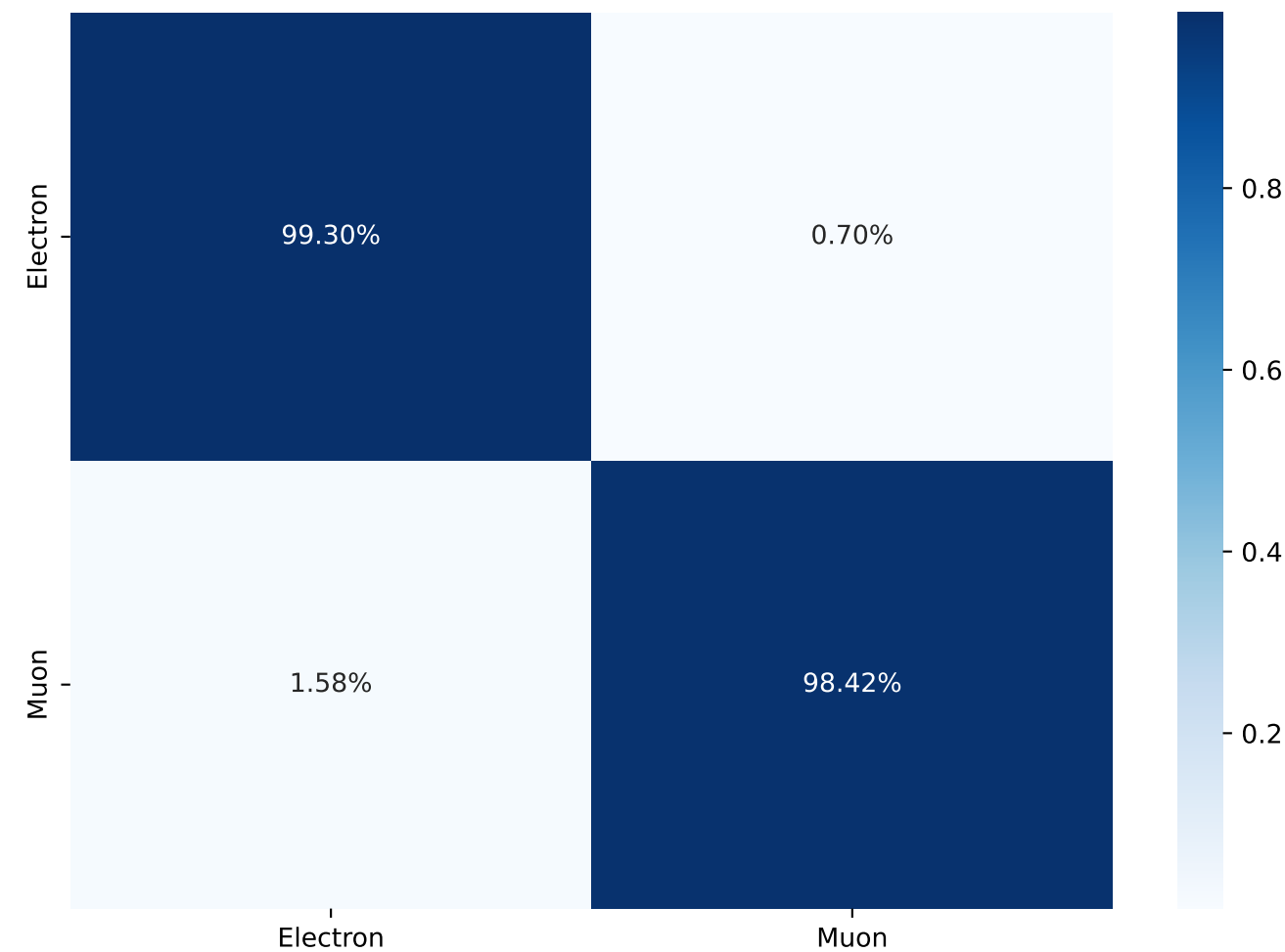
Classifier Response
