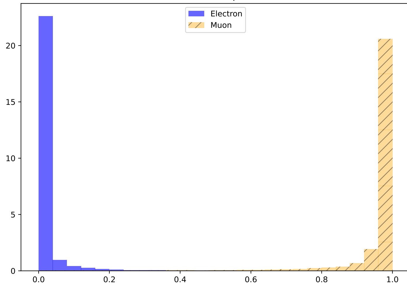
Classifier Response
